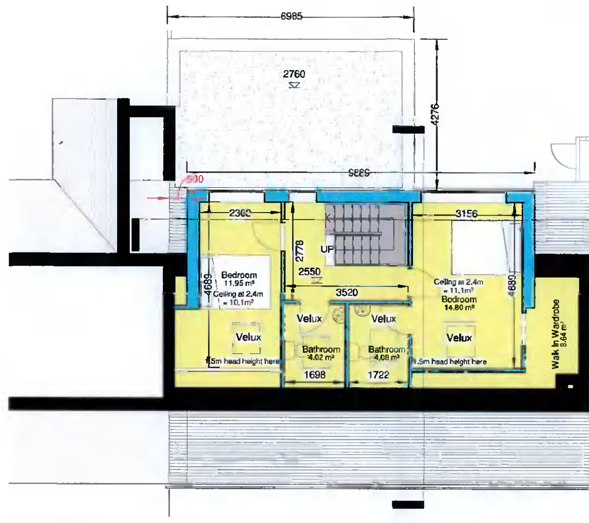
Proposed Attic Plan 1:100
