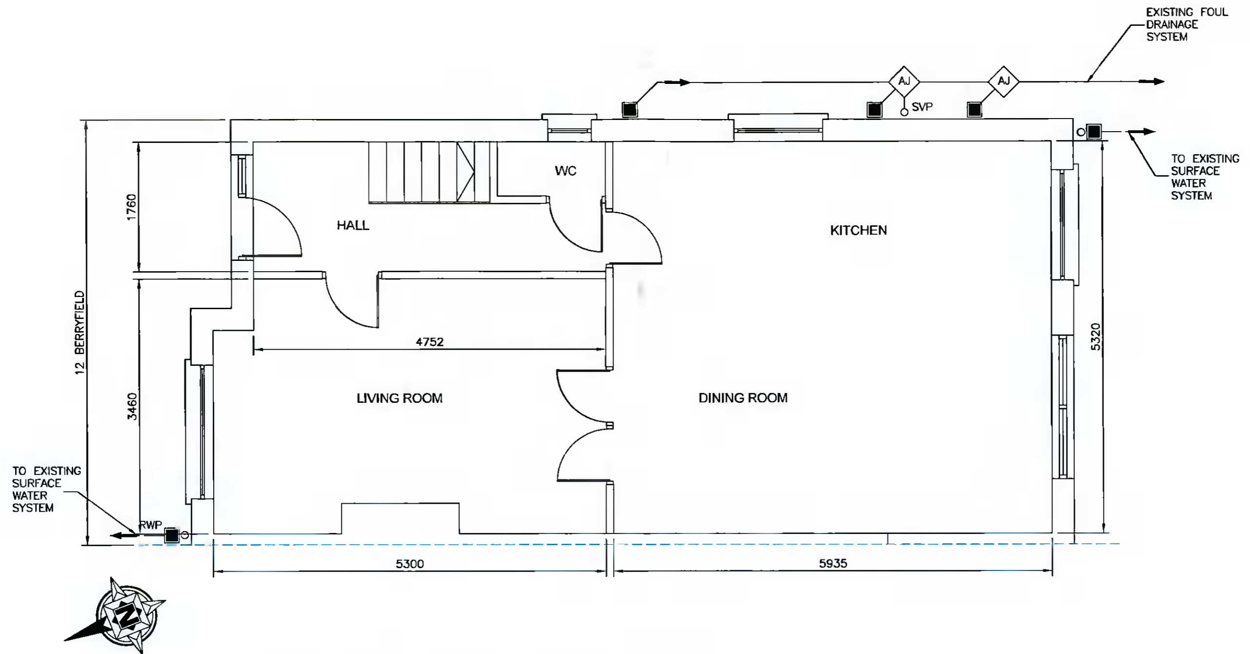
EXISTING GROUND FLOOR PLAN VIEW
