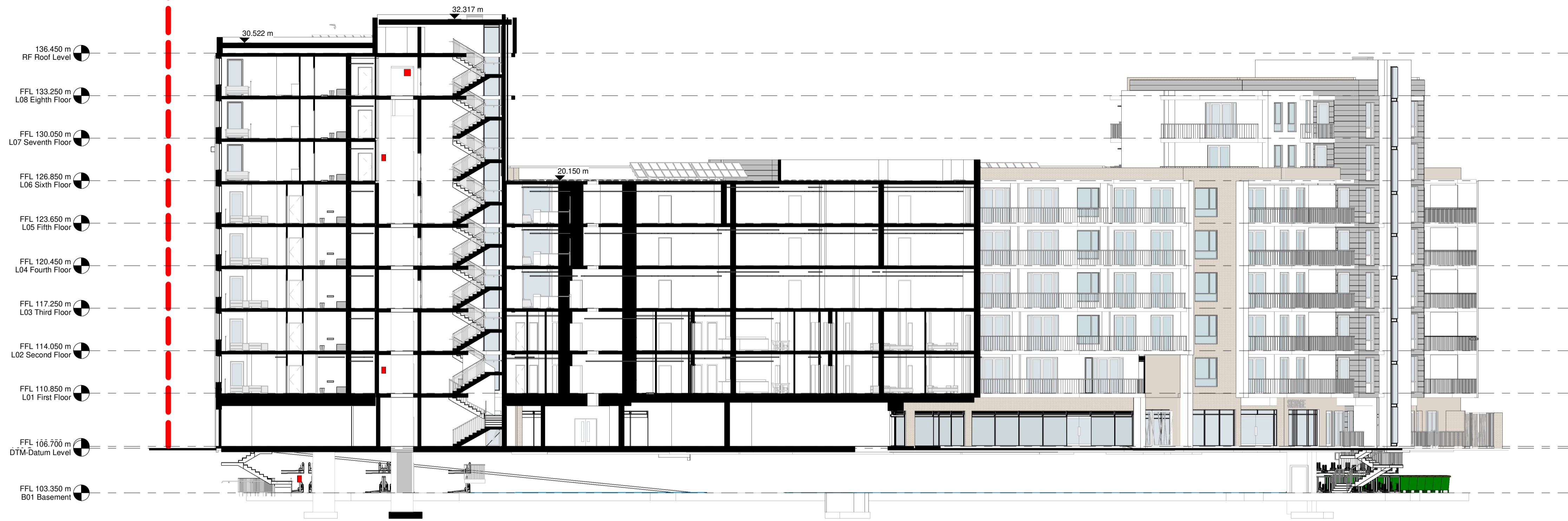
Proposed Section BB 1 : 200
