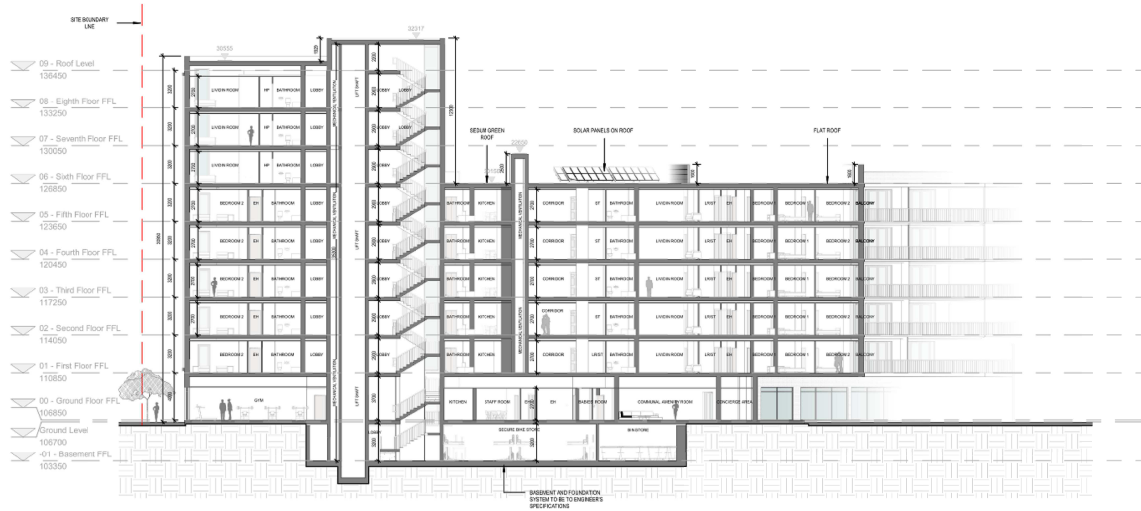
Section BB (Consented) 1:200
