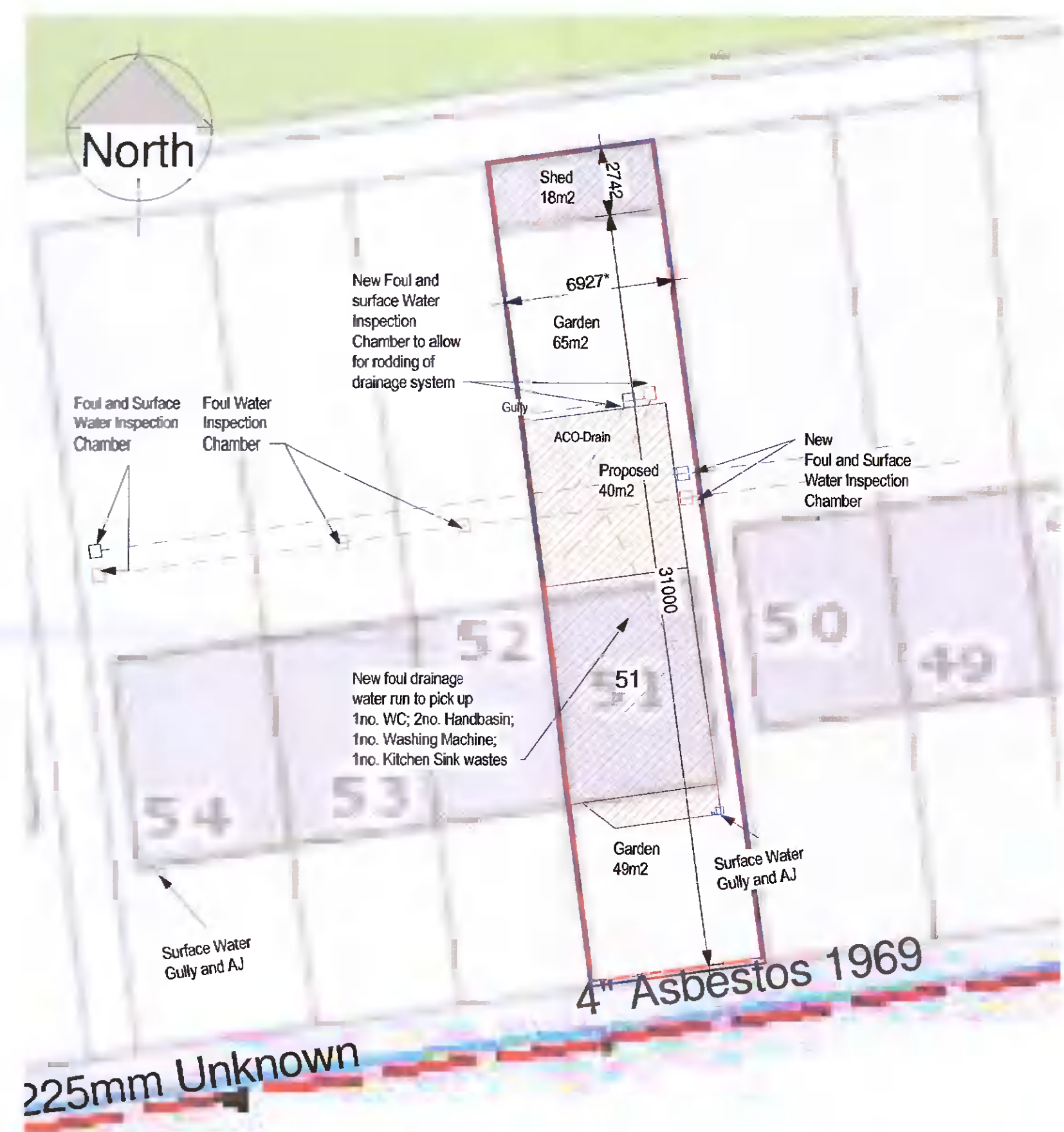
1 51 Airlie Hts Lucan_Watermains & Drainage_Callout 1 : 200
