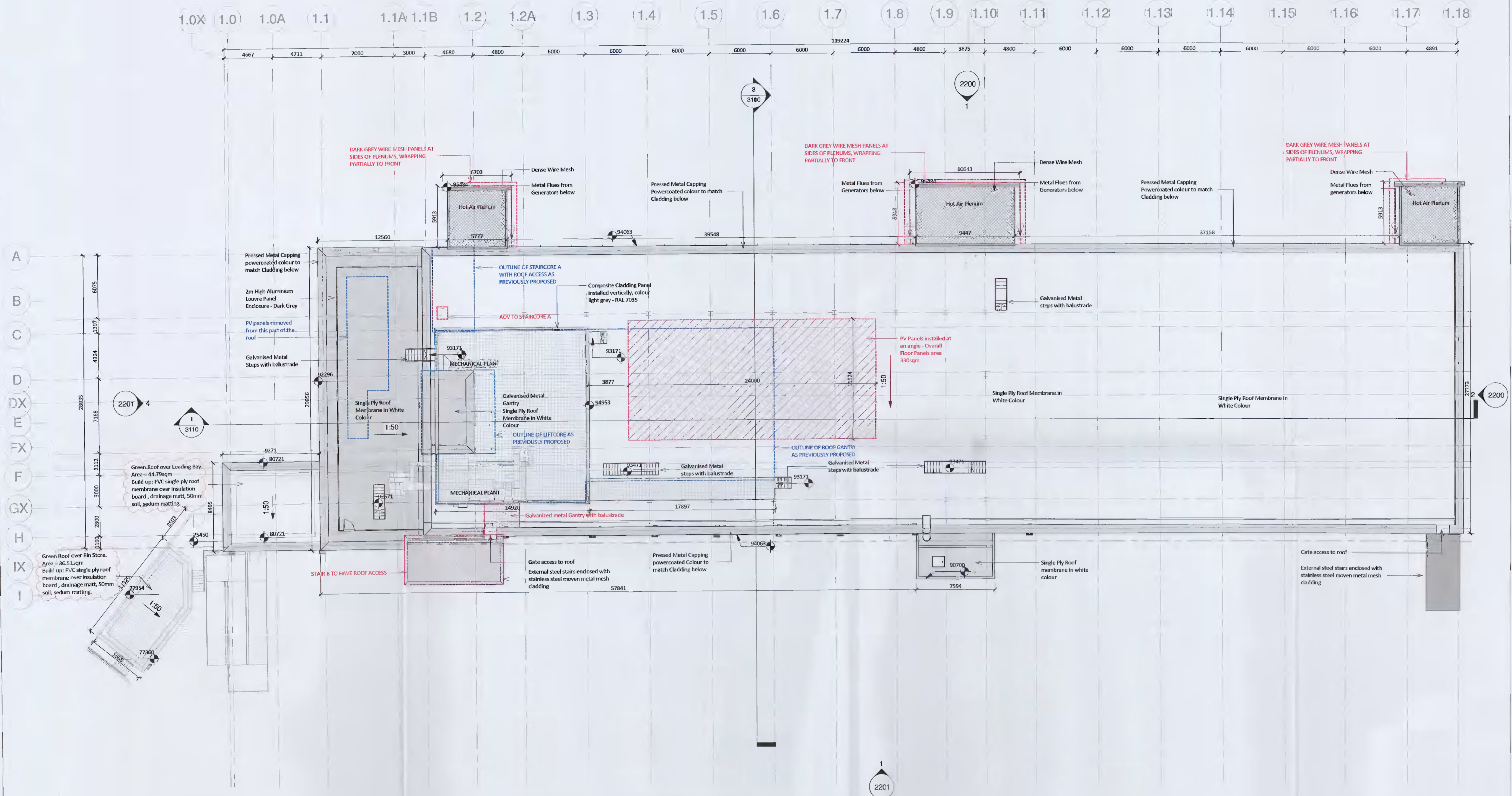
1 05 Overall Roof Level 1 : 200
