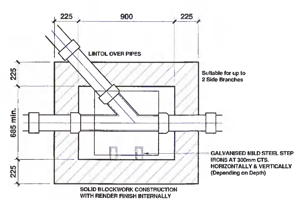
TYPICAL MANHOLE DETAIL - for Manholes & Pipework less than 1.5m deep
