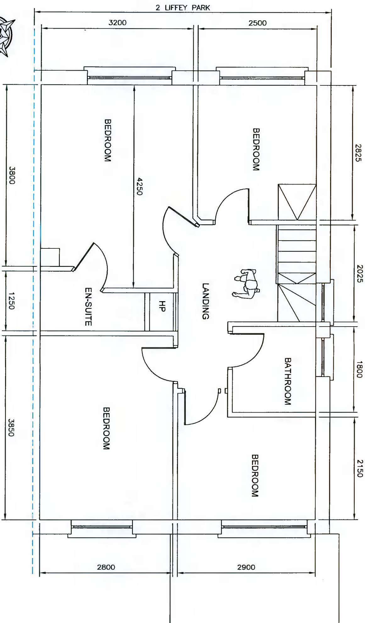
EXISTING FIRST FLOOR PLAN VIEW
