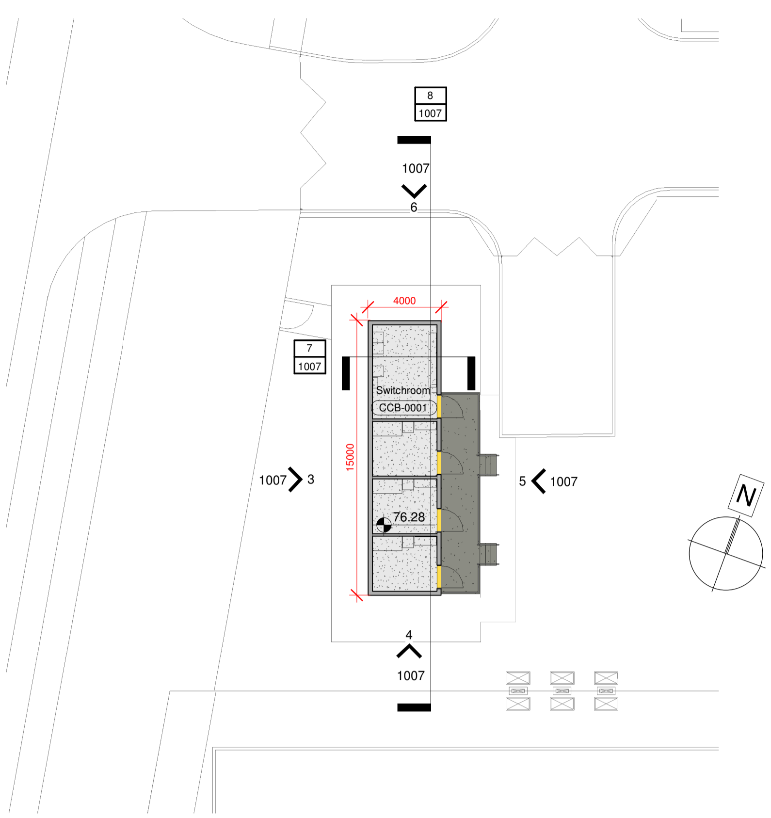
1 1007 Ground Floor Level 1 : 200
