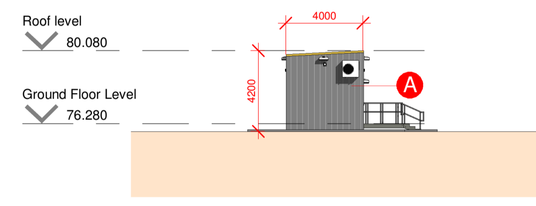
4 1007 South Elevation 1 : 200
