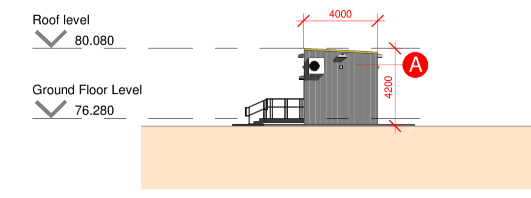
6 1007 North Elevation 1 : 200
