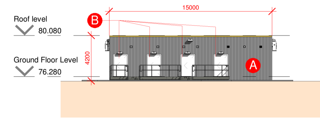
5 1007 East Elevation 1 : 200
