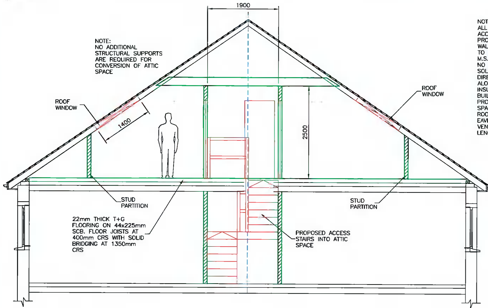
PROPOSED SECTION VIEW
