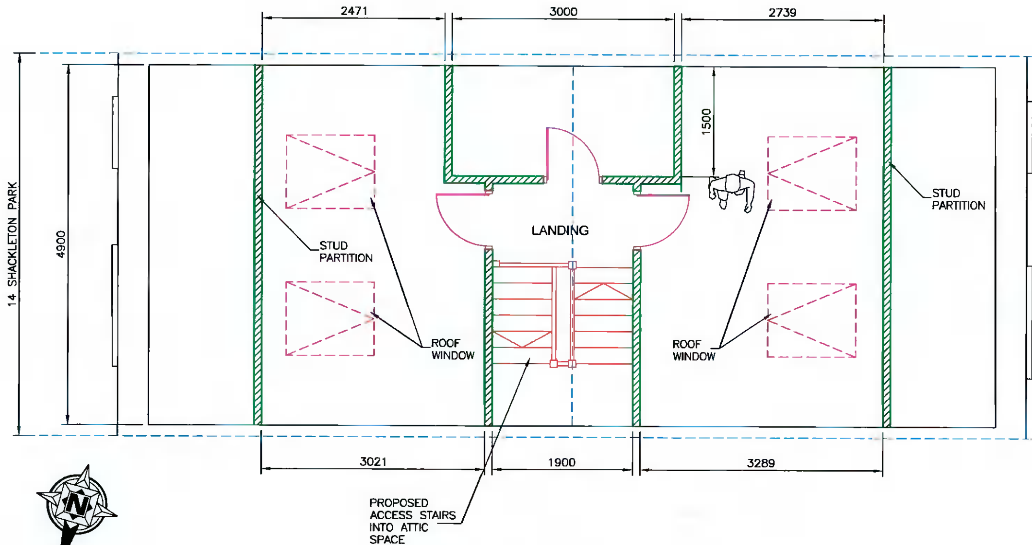
PROPOSED ATTIC FLOOR PLAN VIEW
