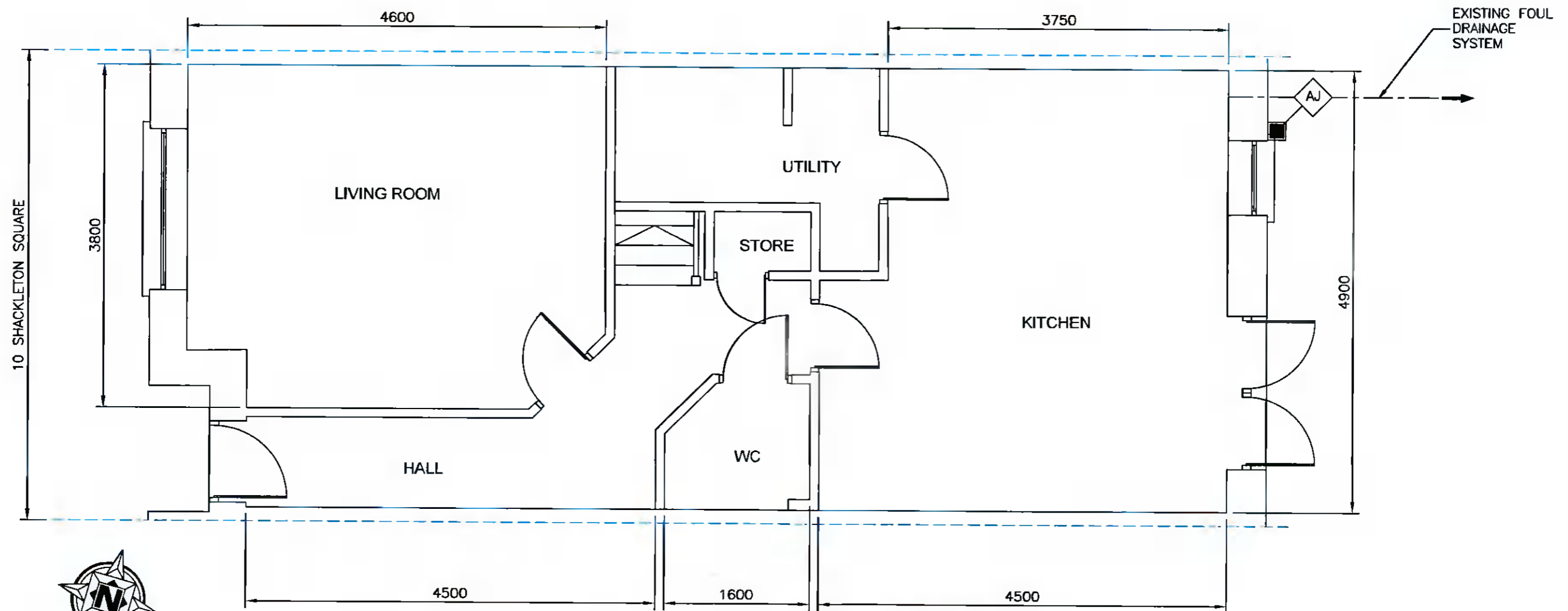
EXISTING GROUND FLOOR PLAN VIEW
