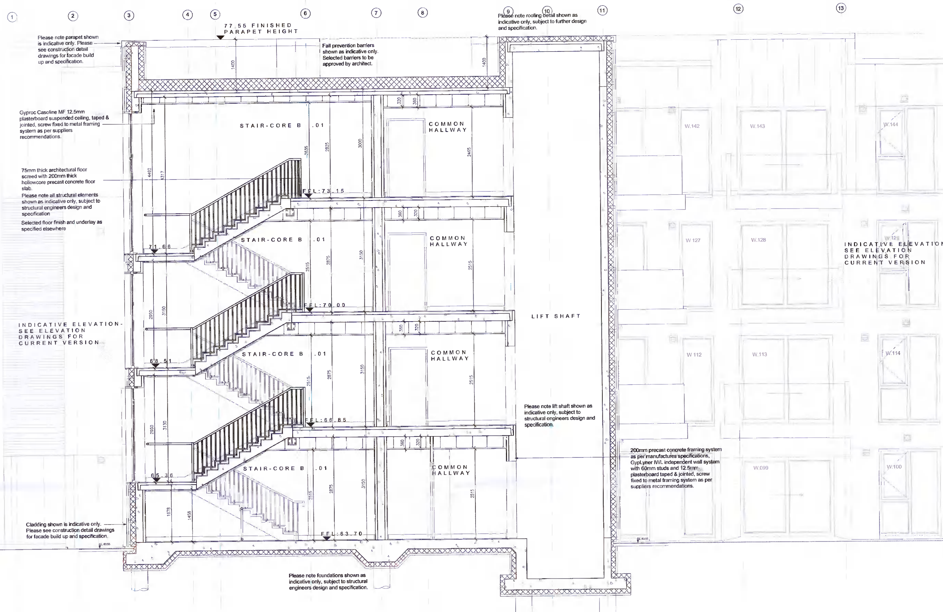
Section G-G - Block B
