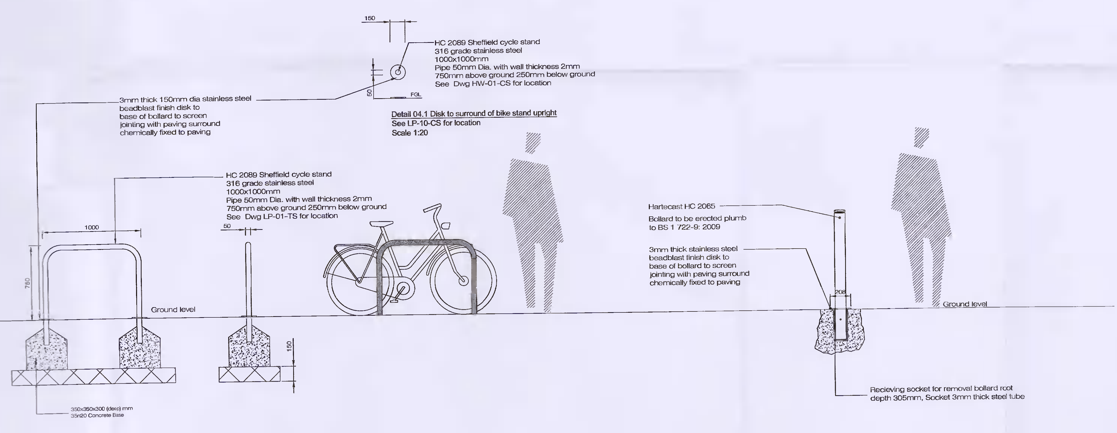
Detail D 04 Drawing LD-03-PP Removable bollards to maintenance access points see LP-01-PP for locations. Scale @ 1:20
