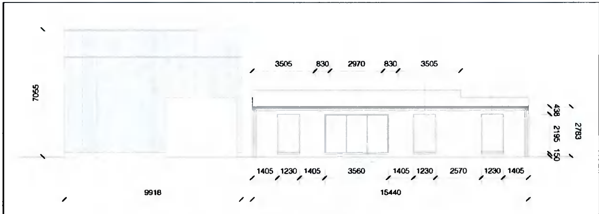
Figure 11.0 North-West elevation of proposed development.
