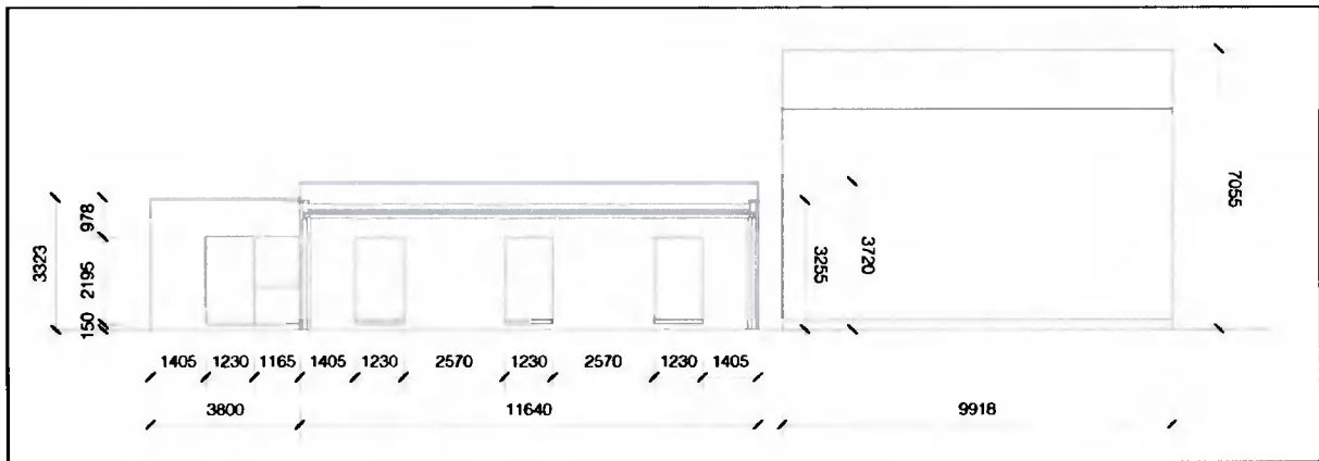
Figure 12.0 South-East elevation of proposed development.
