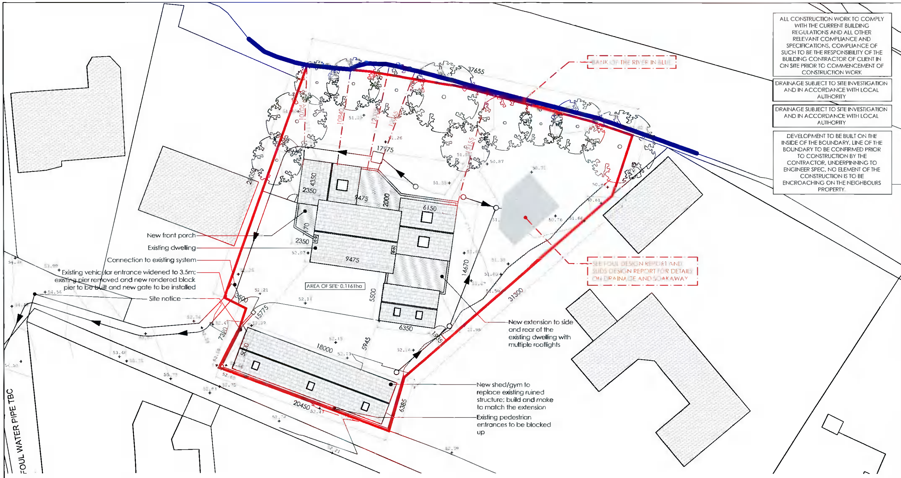
PROPOSED SITE PLAN [LICENCE NO: 50227608 MAP REFERENCE: 3391-01, 3391-02, DN022, x712763y728582] scale 1:250 @ A3
