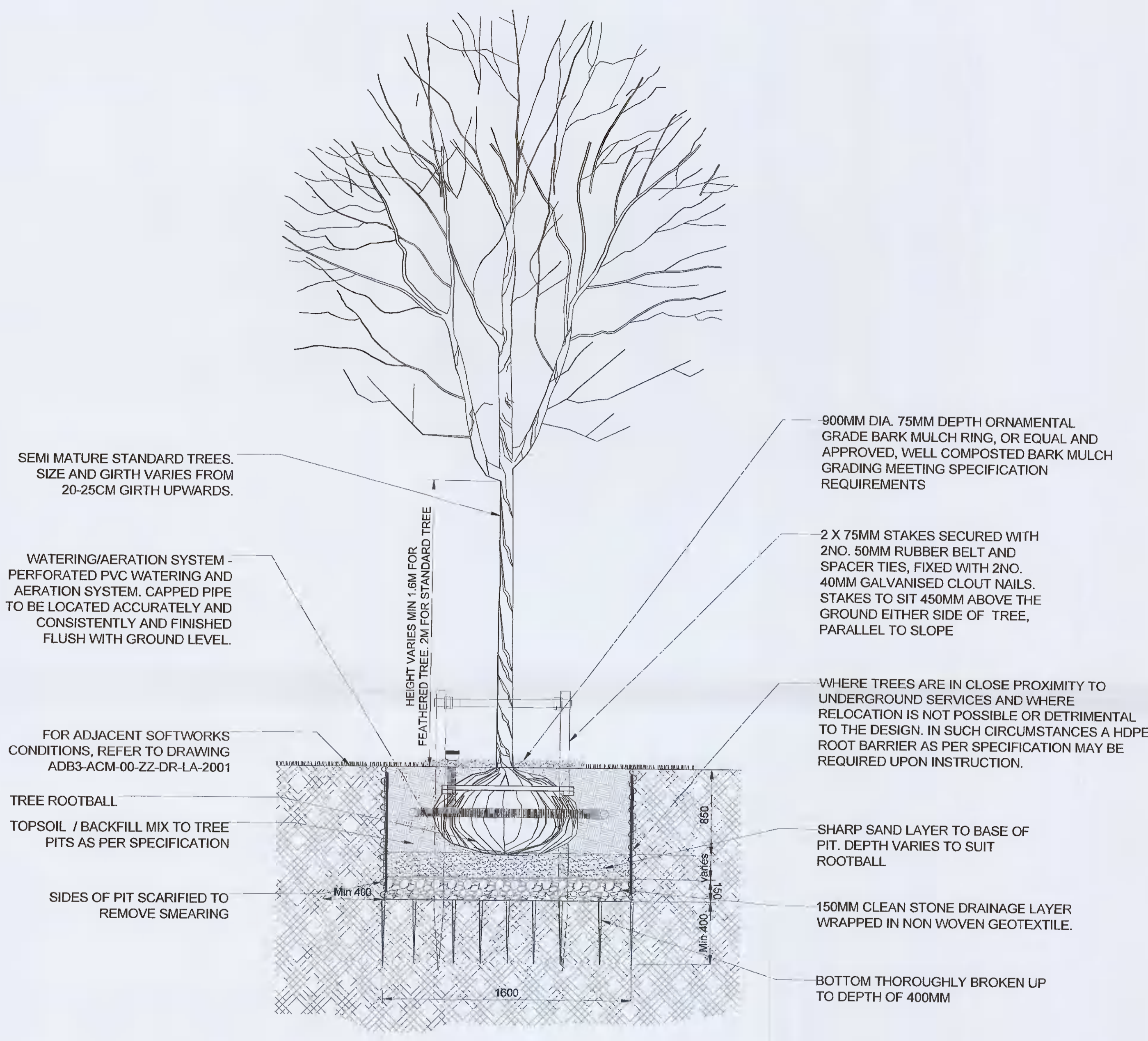
01 SEMI MATURE TREE IN SOFTSCAPE 7200 Scale 1:20@A1
