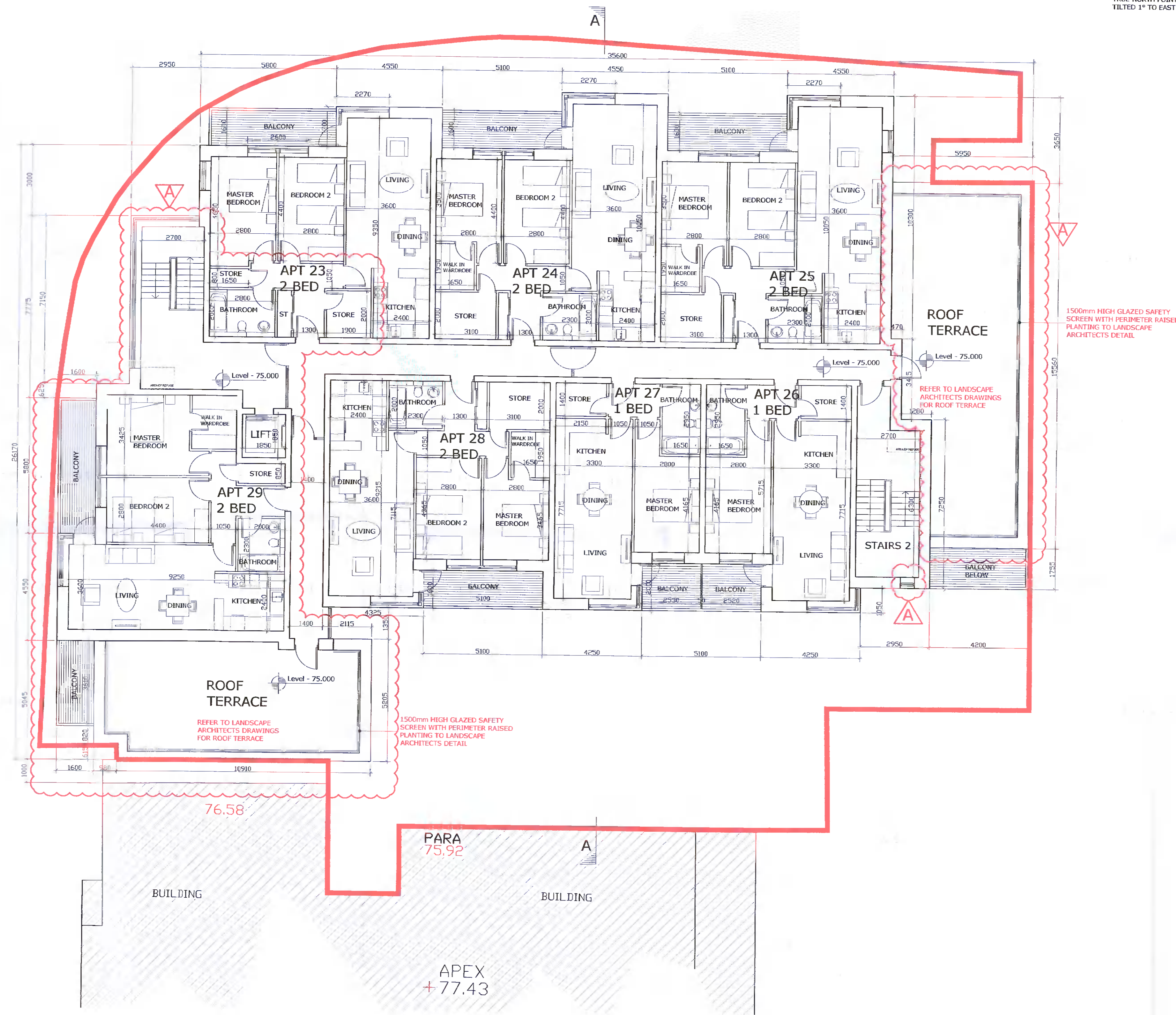
Proposed 3rd Floor Plan Scale 1:100 A1, 1:200 A3
