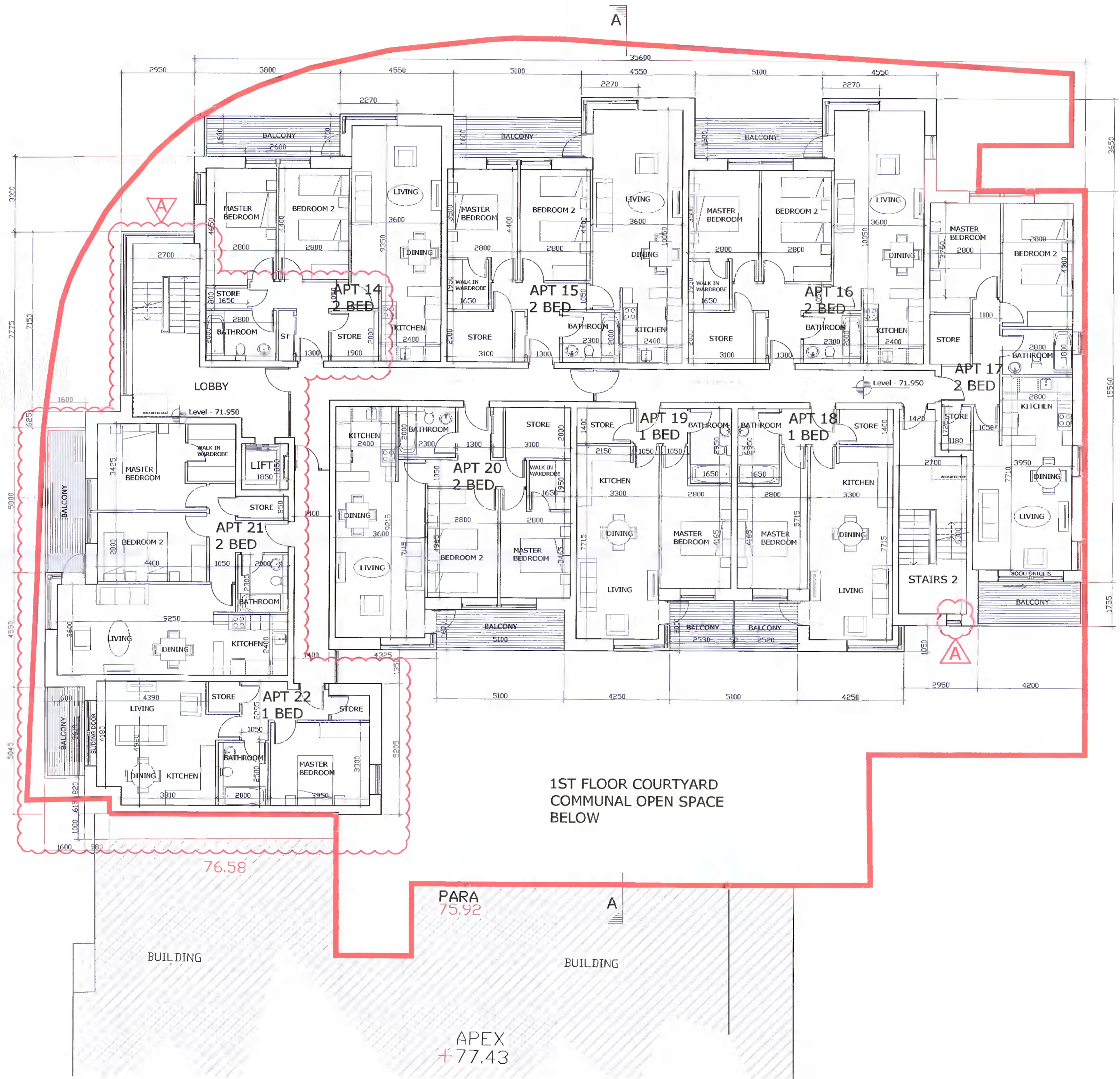
Proposed 2nd Floor Plan Scale 1:100 A1, 1:200 A3
