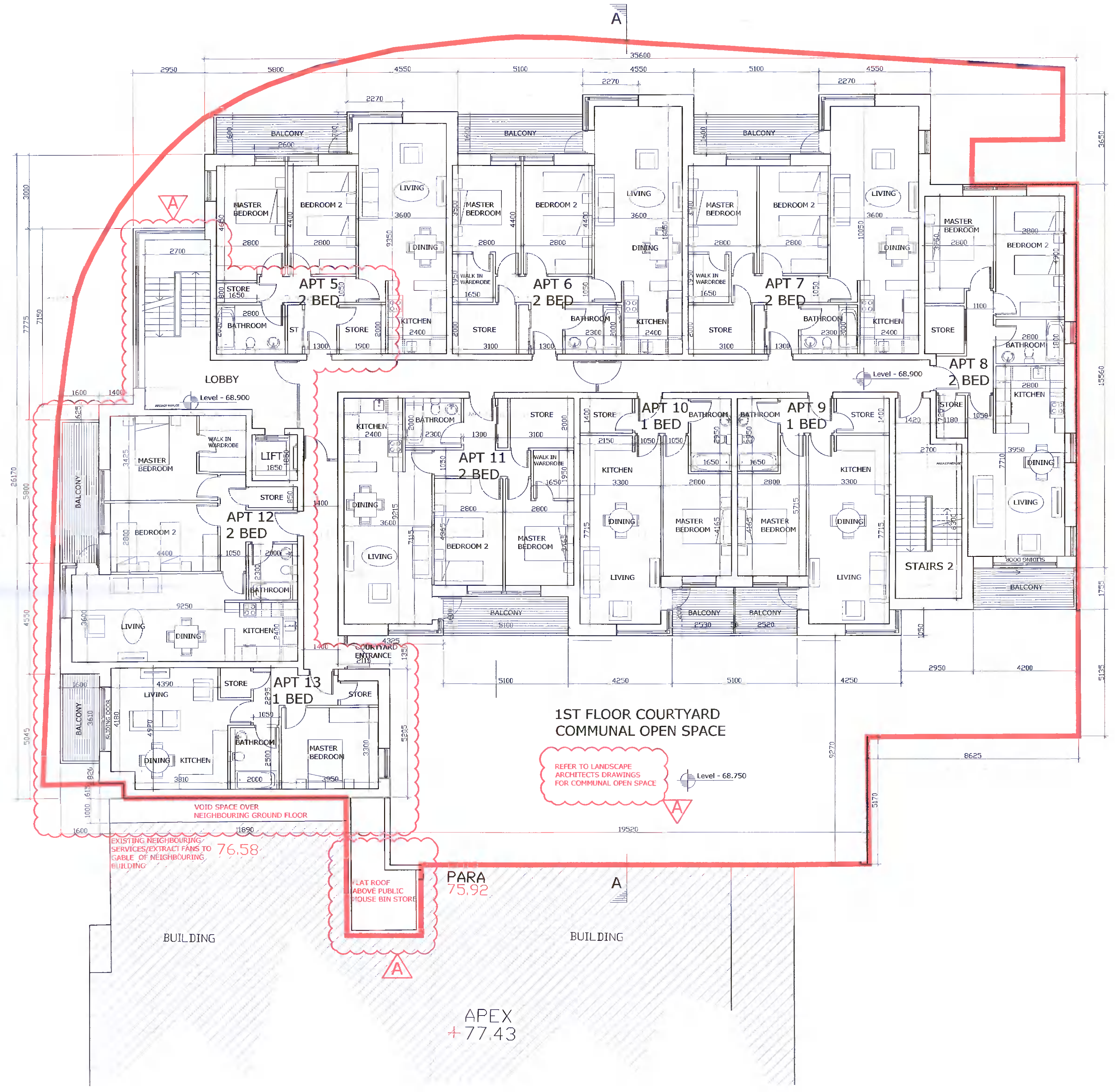
Proposed 1st Floor Plan Scale 1:100 A1, 1:200 A3
