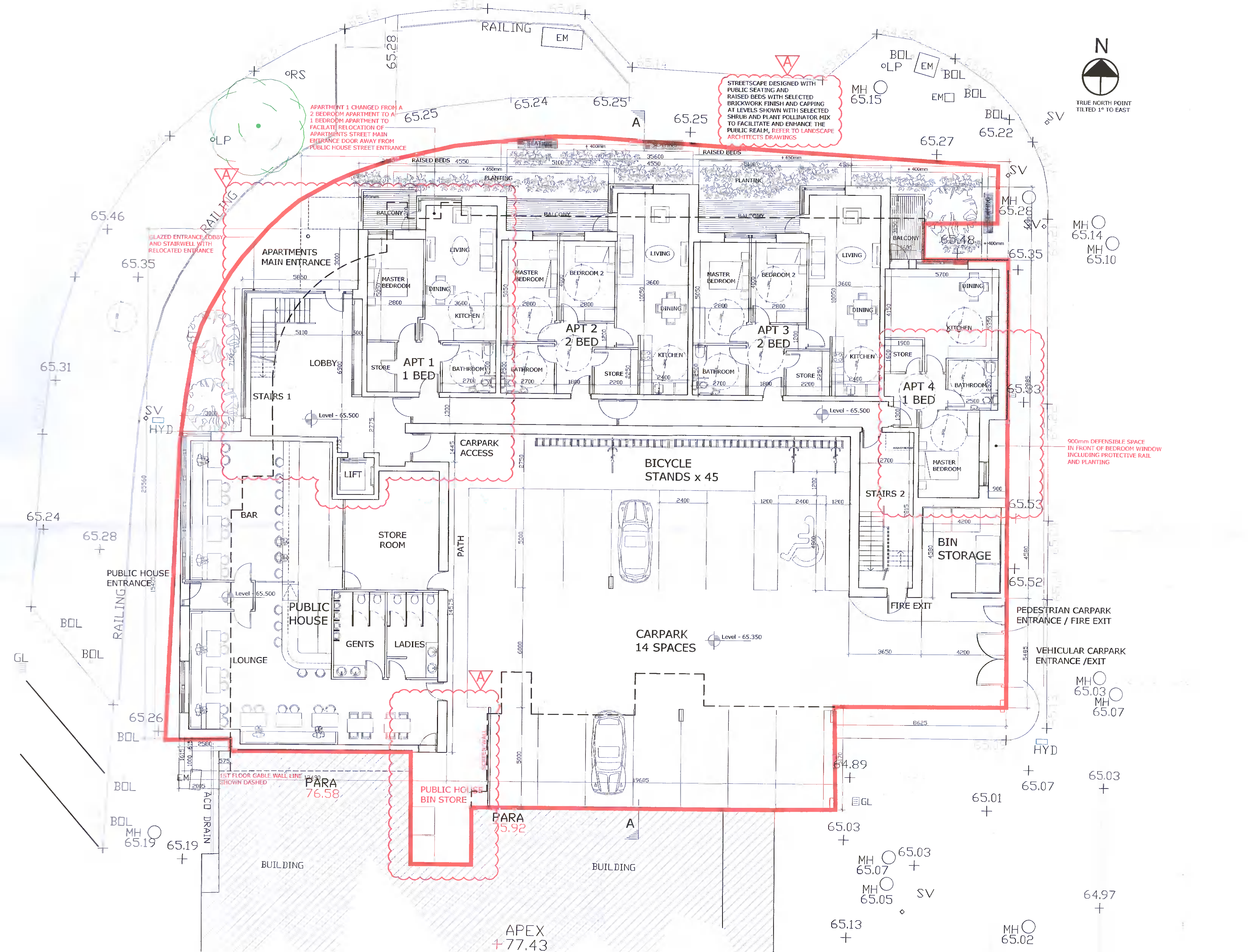
Proposed Ground Floor Plan Scale 1:100 A1, 1:200 A3
