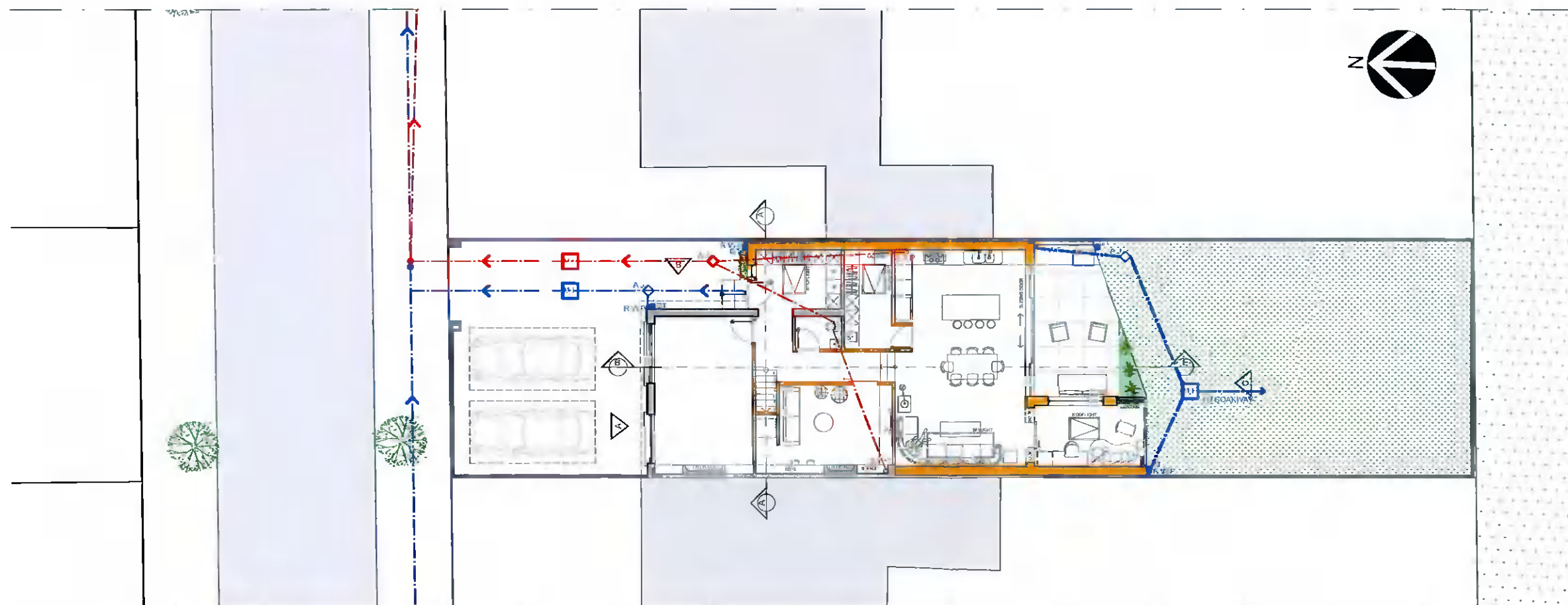
O2 PROPOSED DRAINAGE PLAN SCALE: 1:200
