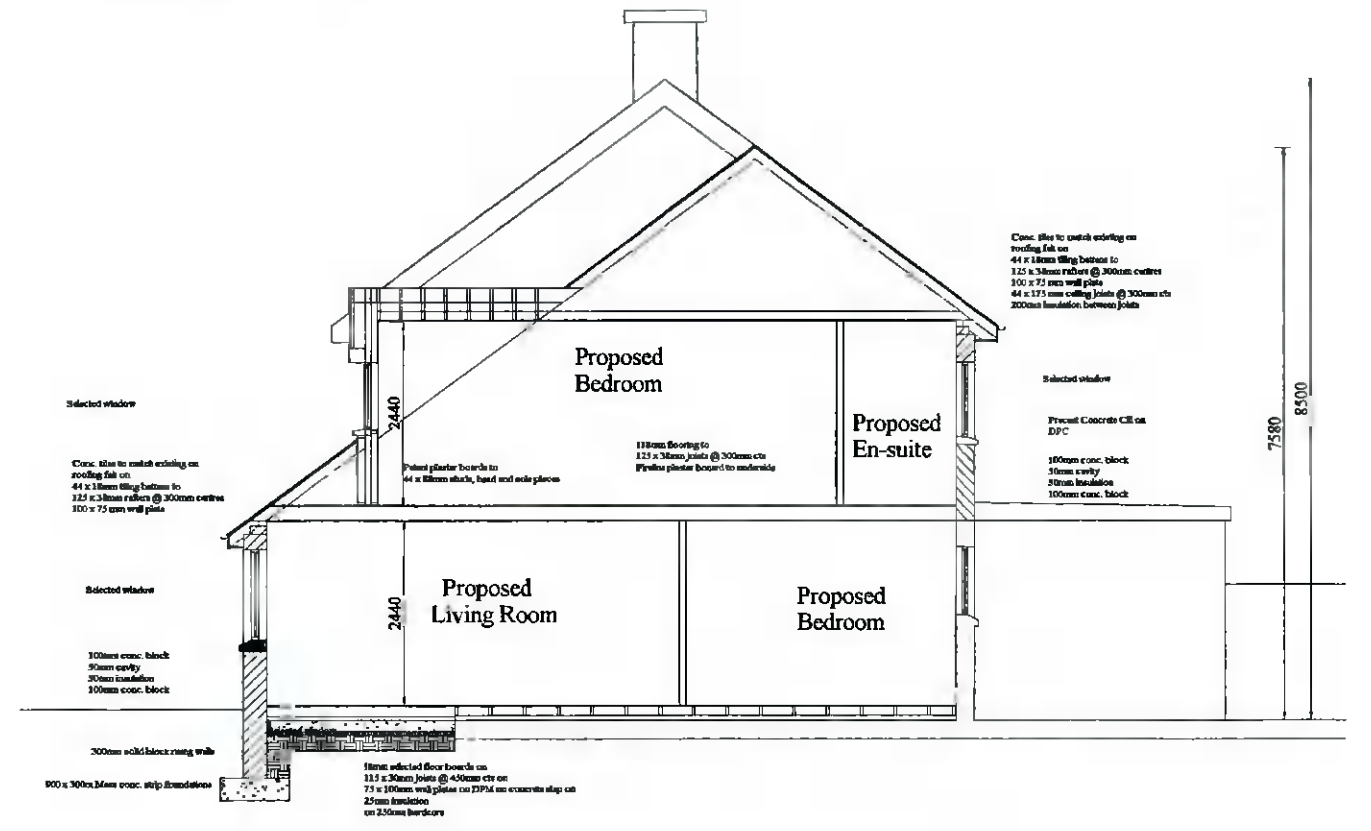
Section XX
