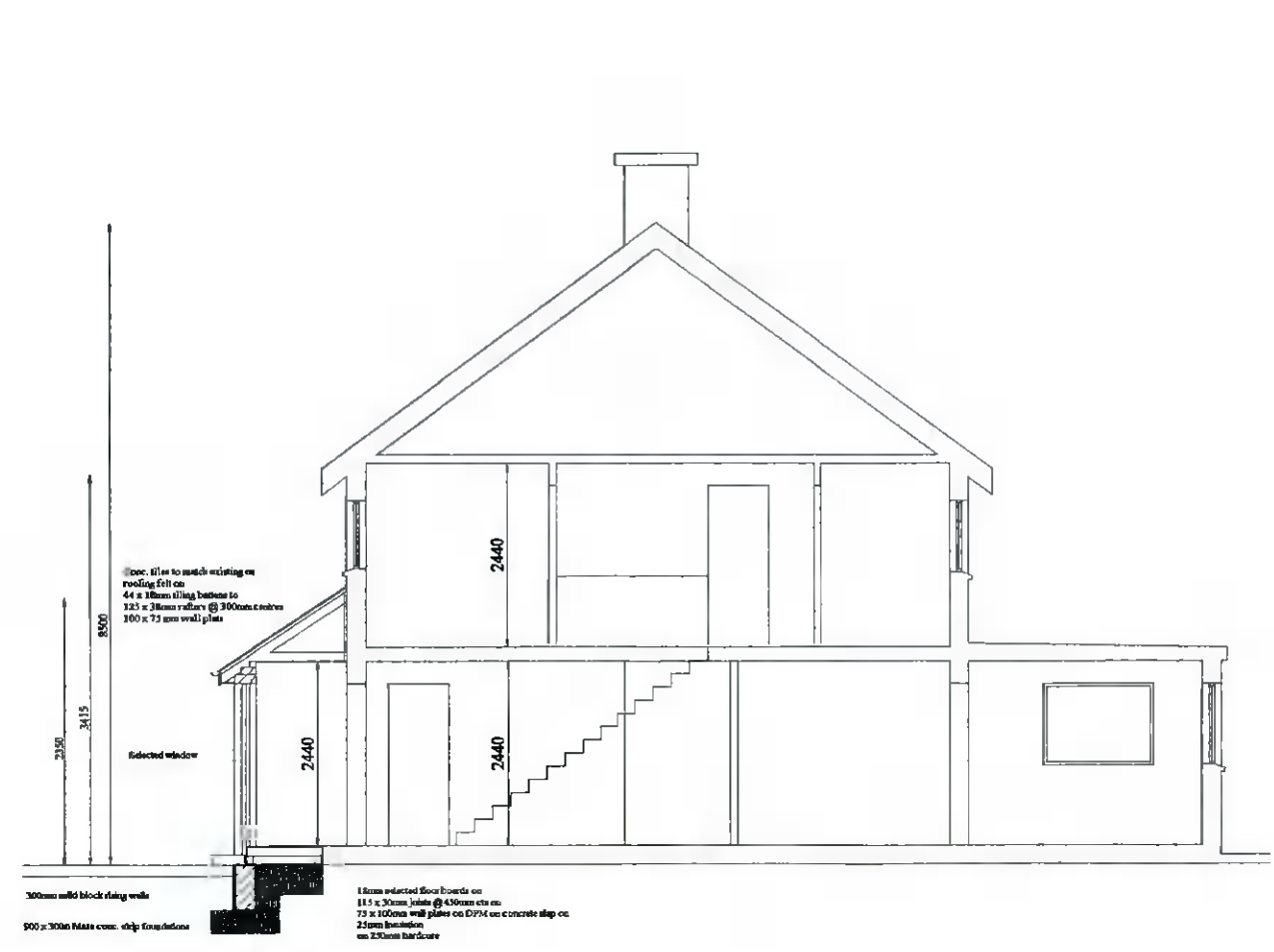
Section YY
