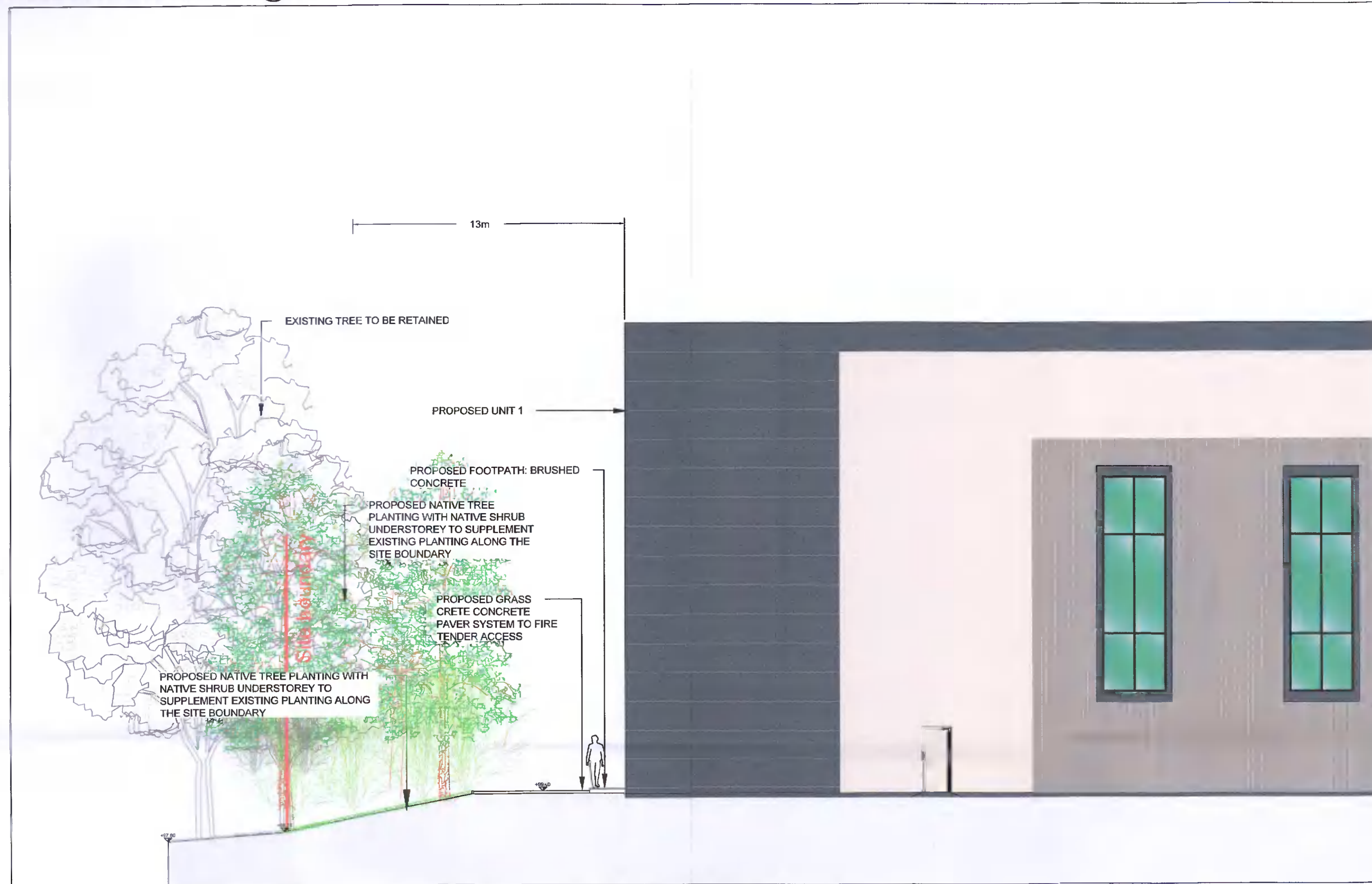
Section E-E scale 1:100@A1
