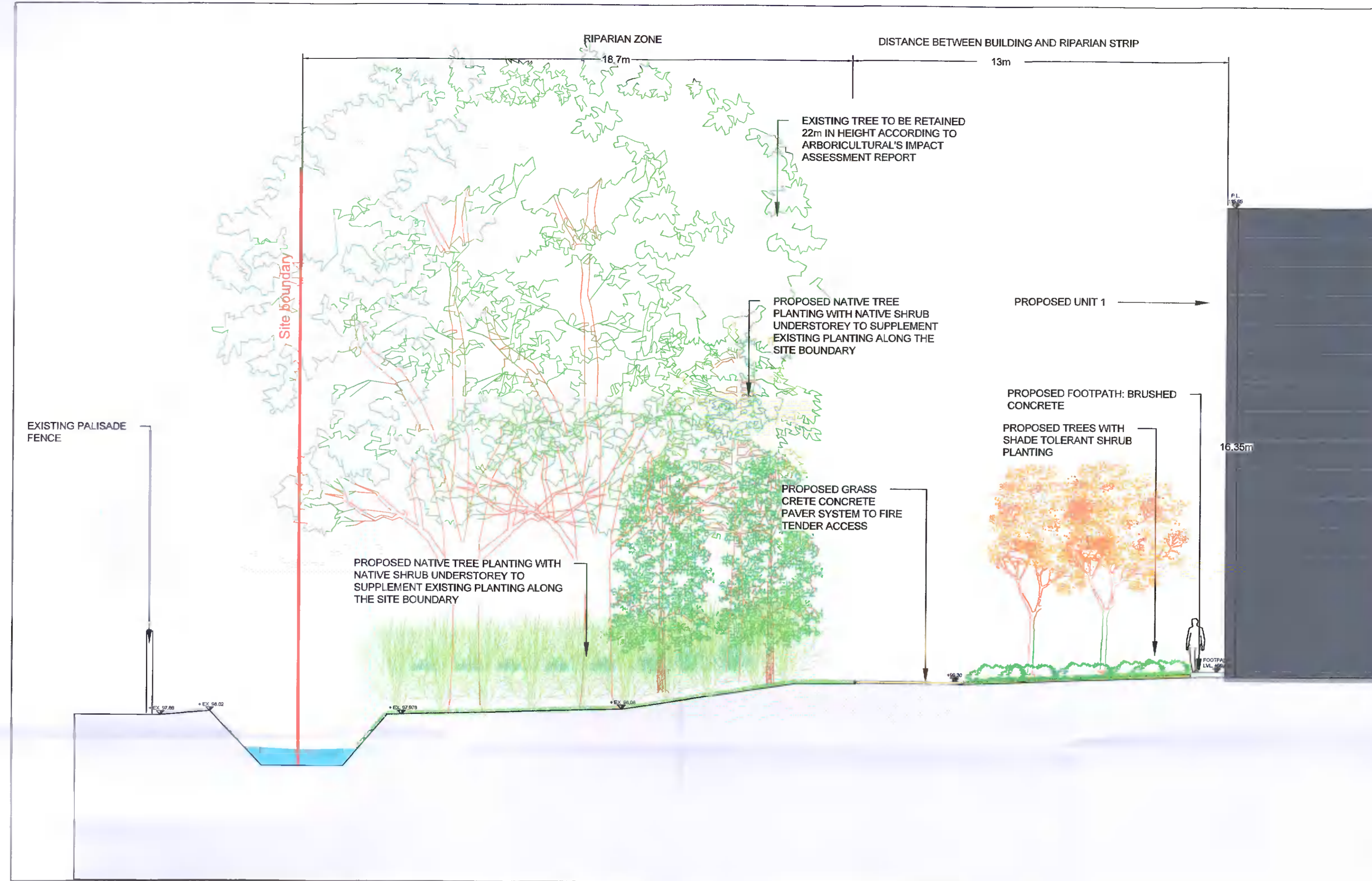
Section C-C scale 1:100@A1
