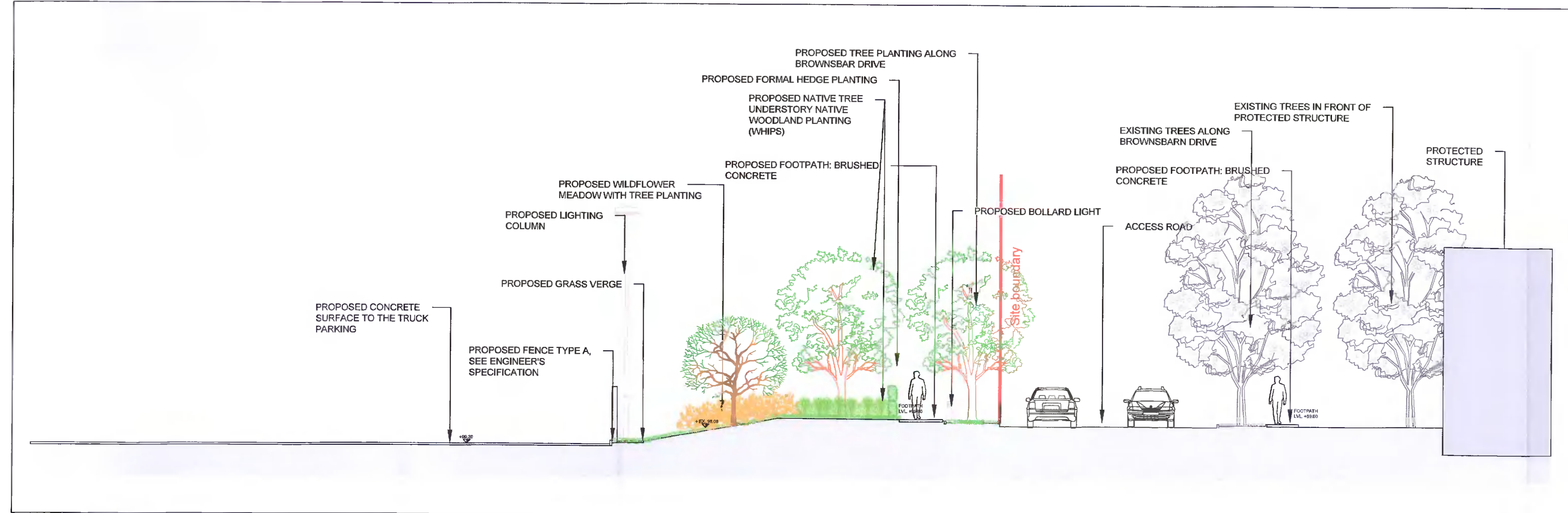
Section D-D scale 1:100@A1
