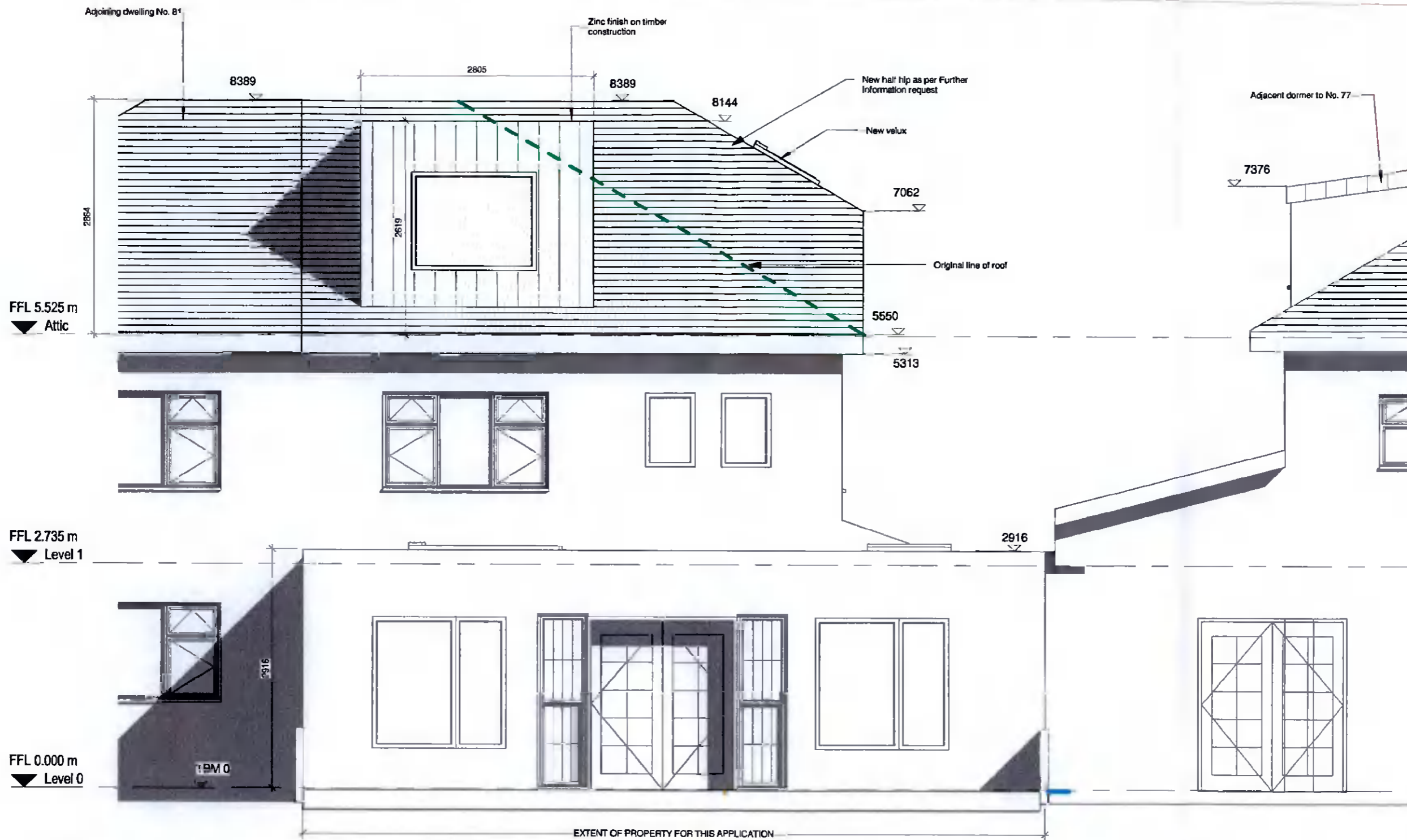
1. Proposed Rear Elevation (East) 1 : 50
