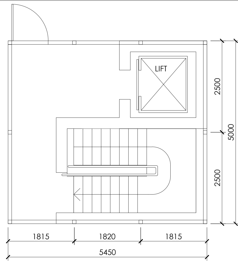
PROPOSED FLOOR PLAN 1:50
