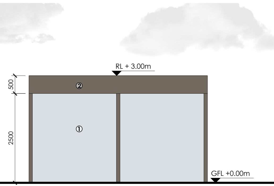
SIDE ELEVATIONS 1:50
