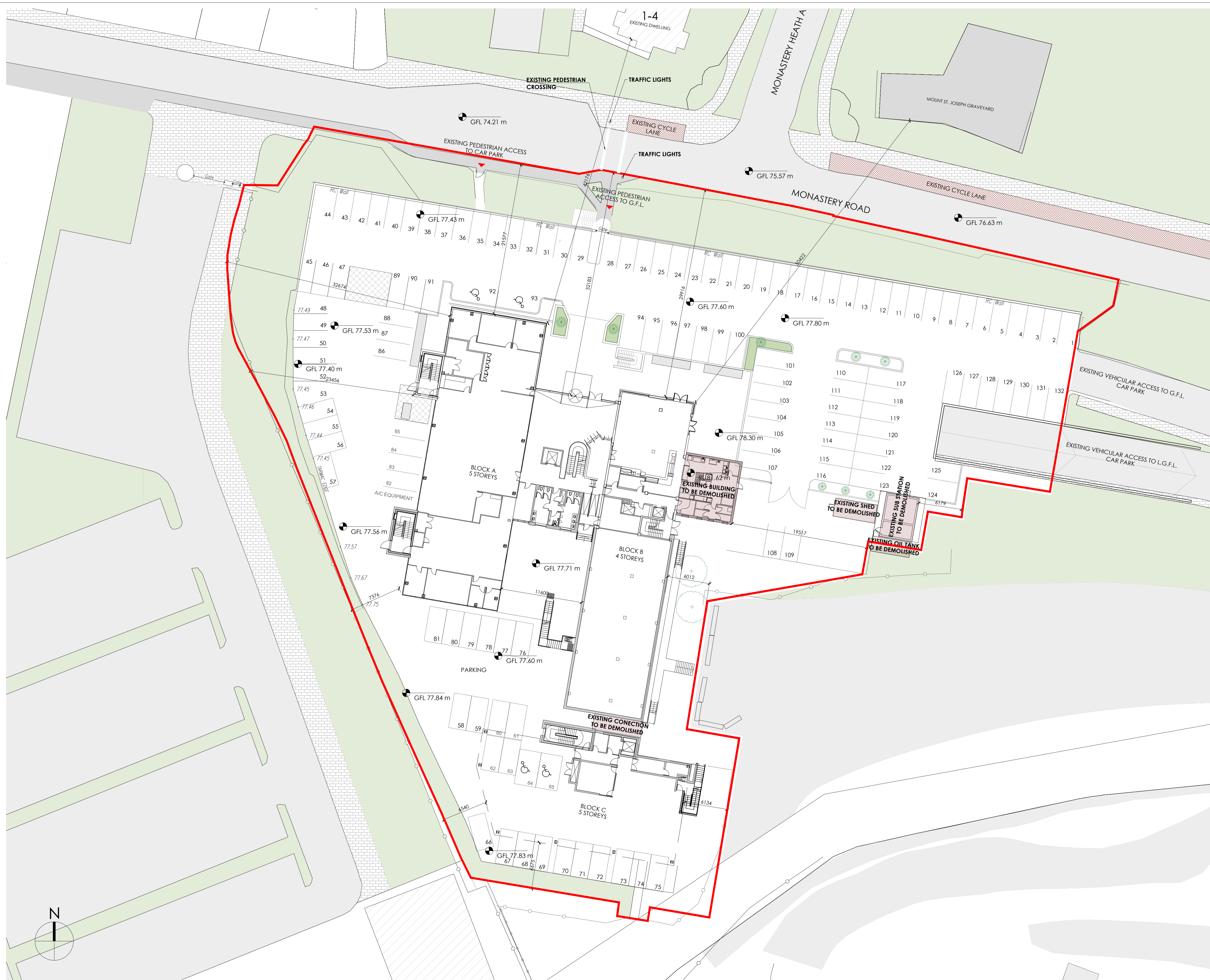
EXISTING/DEMOLITION/REMOVAL WORKS SITE LAYOUT PLAN 1:250
