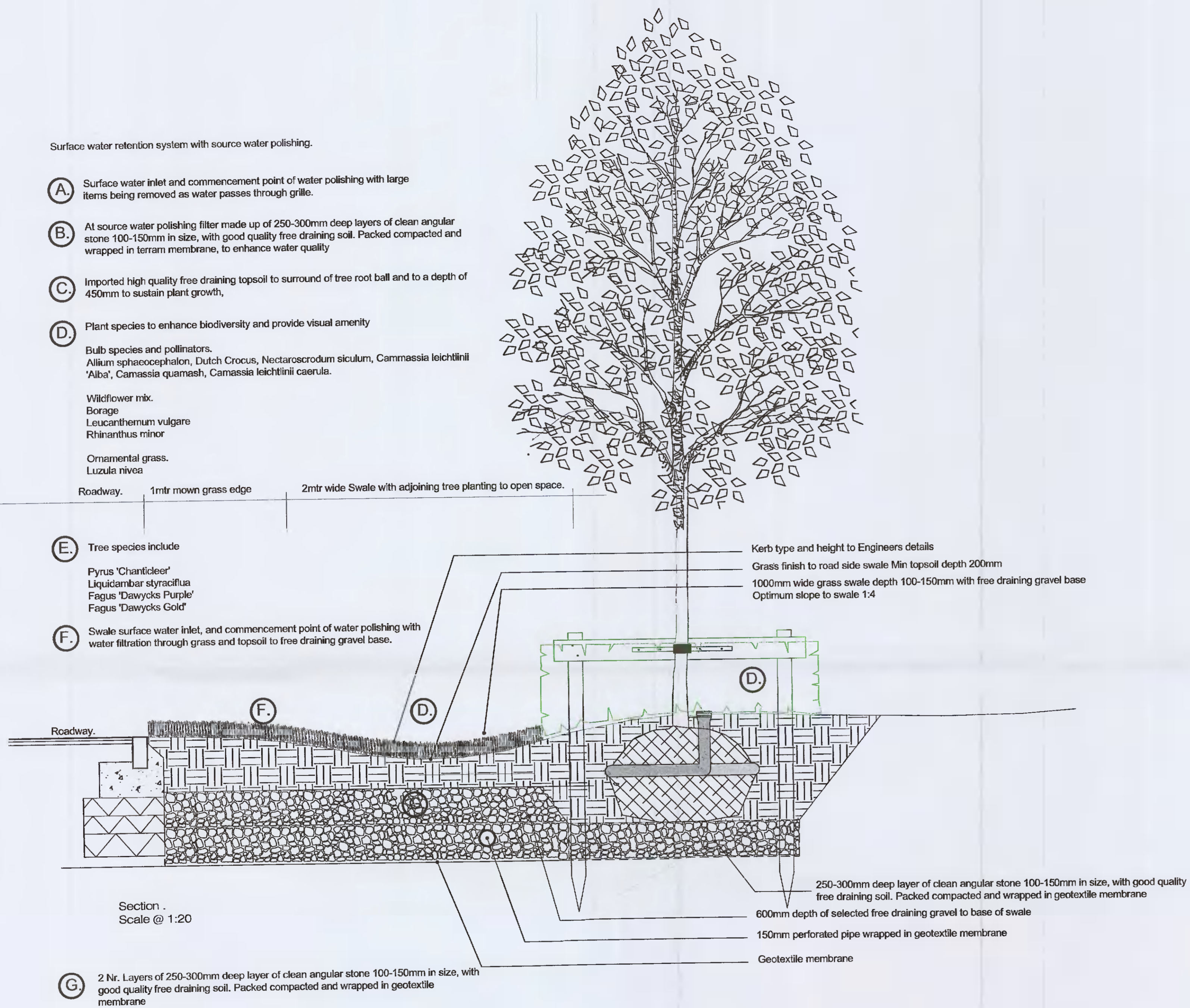
D 01 LD-02-CFI Grass Swale. Scale @ 1:20
