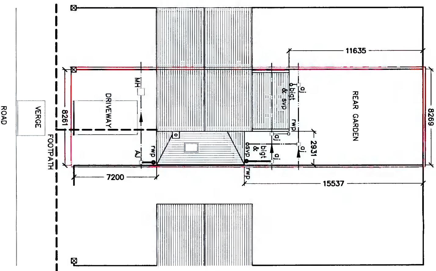
⊕ PROPOSED BLOCK PLAN & DRAINAGE LAYOUT SCALE 1:200
