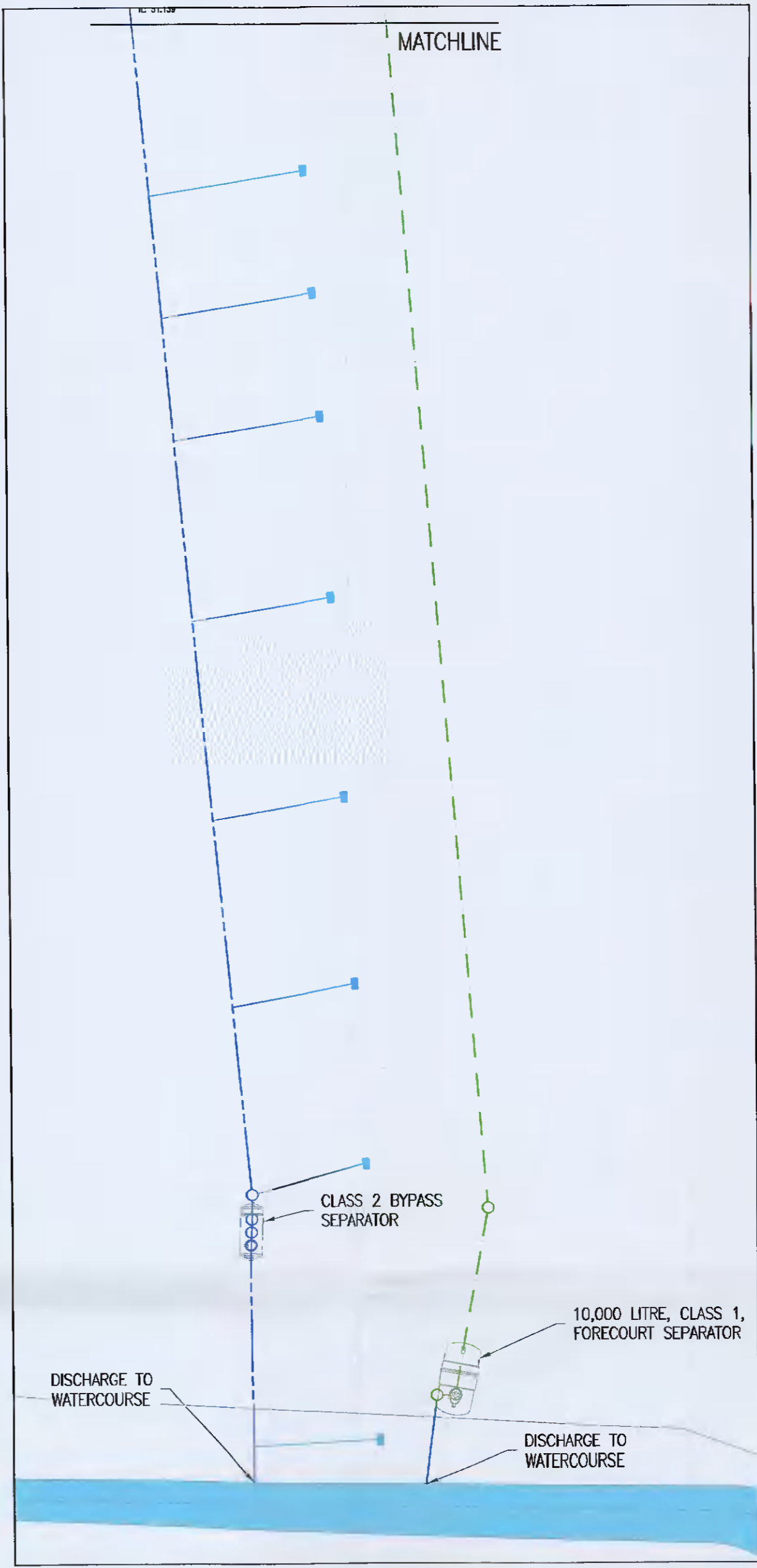
INTERCEPTOR AND DISCHARGE TO WATERCOURSE SCALE 1:250
