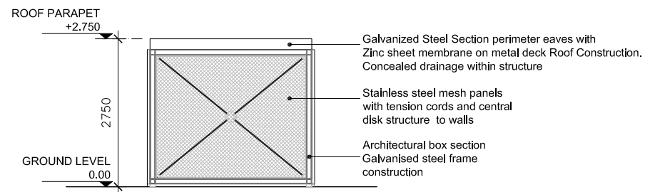
05 Elevation 04 of Bin Store C PA-401 1:100
