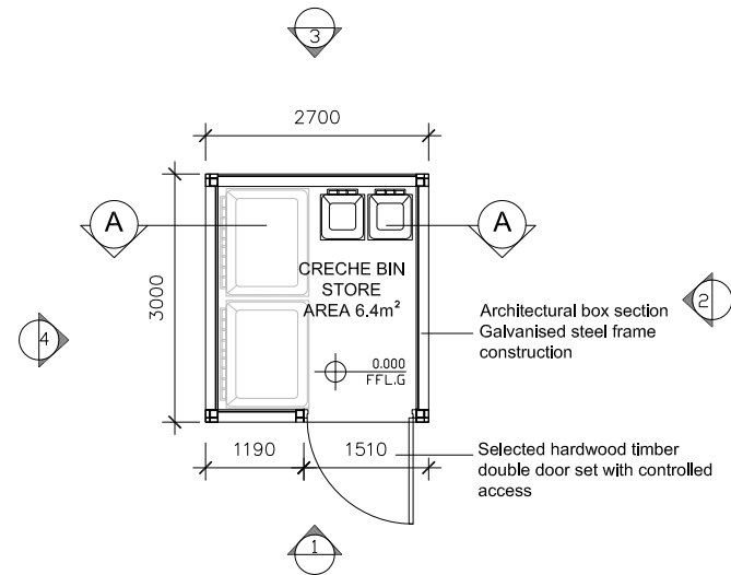
01 Plan of Bin Store C PA-402 1:100
