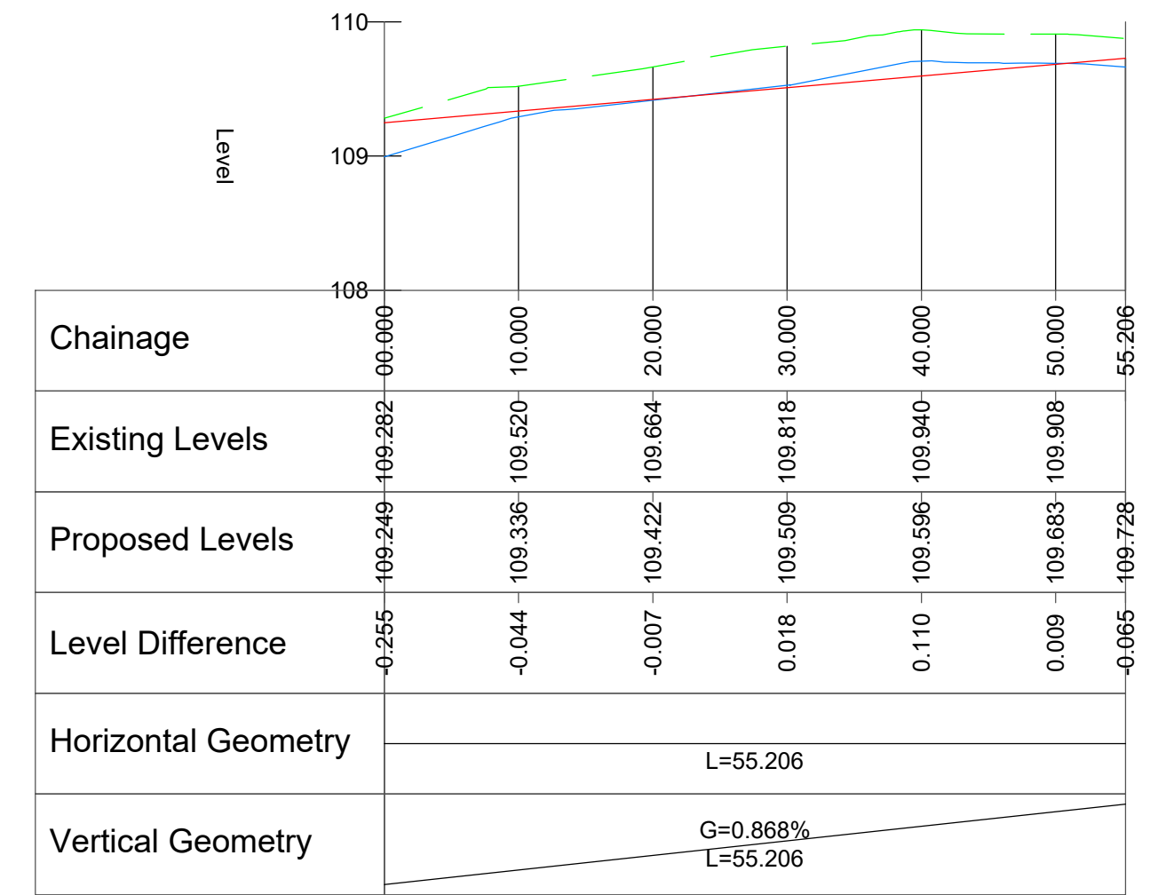
ROAD 3 ALIGNMENT - LONGSECTION SCALE: H 1:500, V 1:50. DATUM: 108.000
