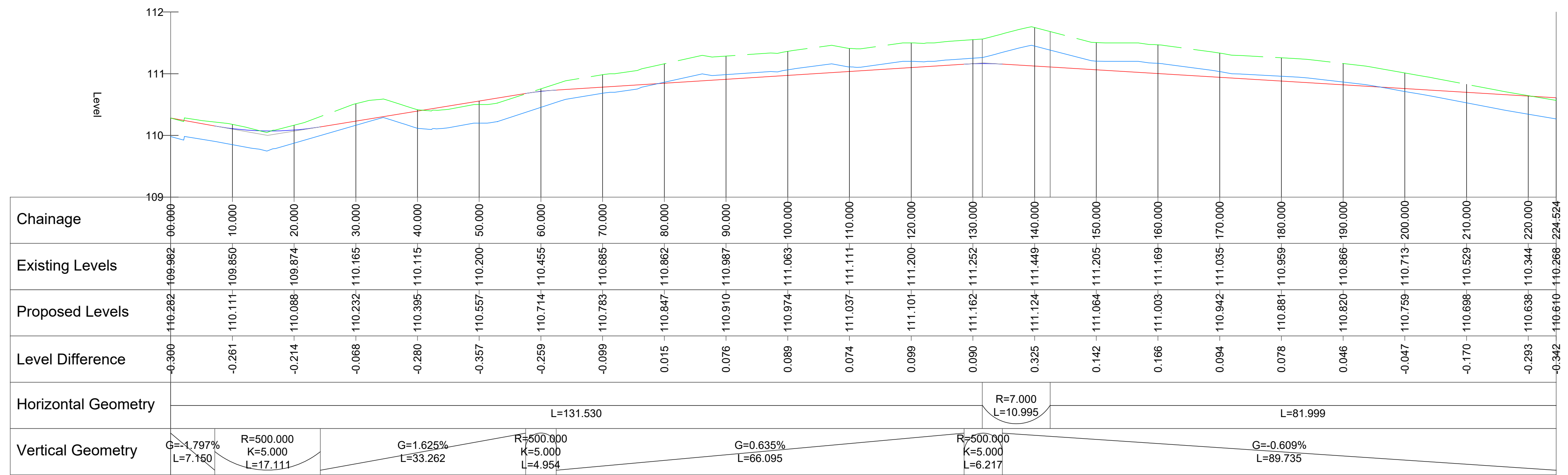
ROAD 1 ALIGNMENT - LONGSECTION SCALE: H 1:500, V 1:50. DATUM: 109.000
