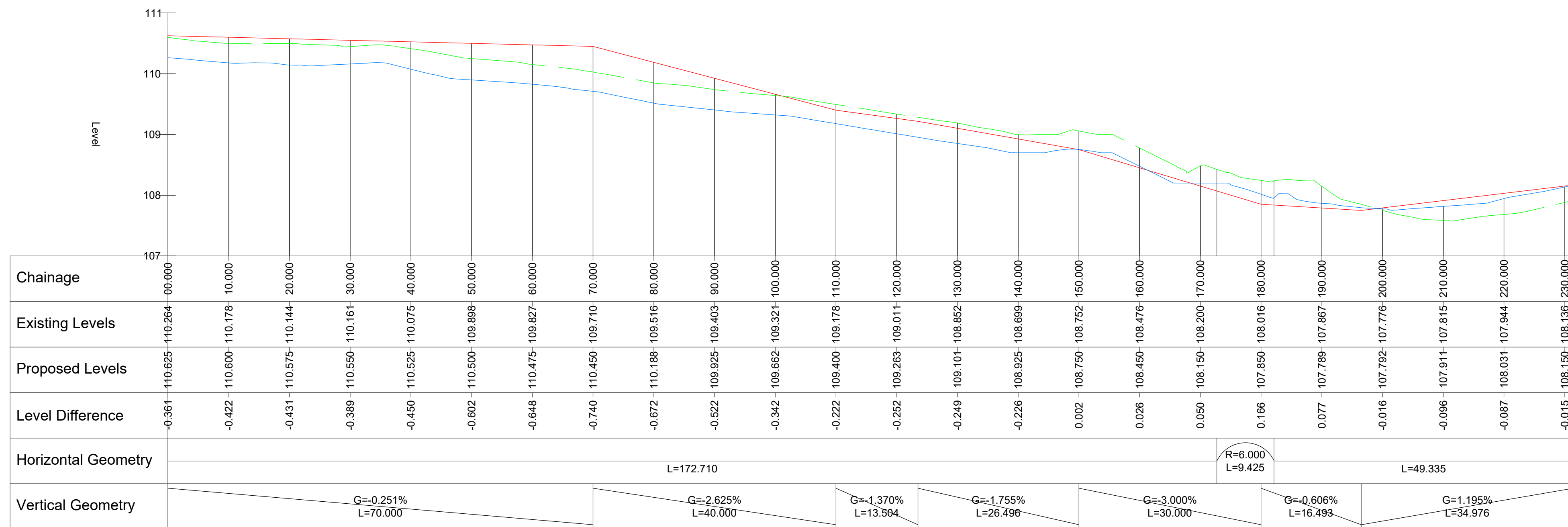
ROAD 2 ALIGNMENT - LONGSECTION SCALE: H 1:500, V 1:50. DATUM: 107.000
