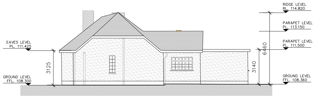
02 South-West Elevation EX-100 1:200
