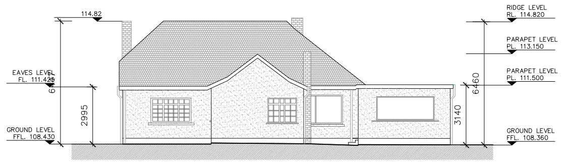
04 South-East Elevation EX-100 1:200
