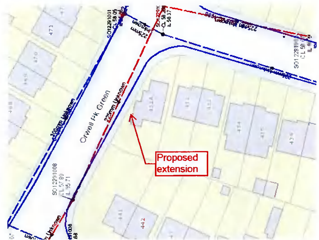
Figure 3:- Extract from drainage record maps
