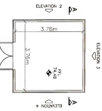
FLOOR PLAN (Scale 1:100)
