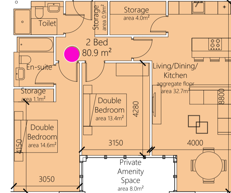
2 BED 4 PERSON i.e. C.1.7 C.2.14 C.3.22 C.4.30 TYPE: 2B4P O2 AREA: 80.9 m 2
