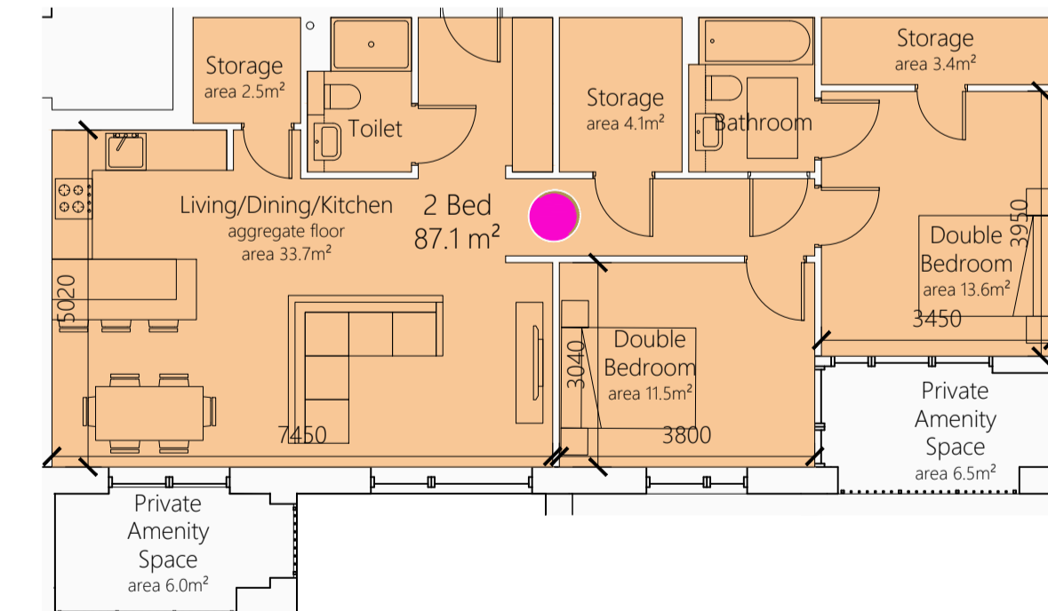
2 BED 4 PERSON i.e. A.8.58 TYPE: 2B4P T1 AREA: 87.1 m 2
