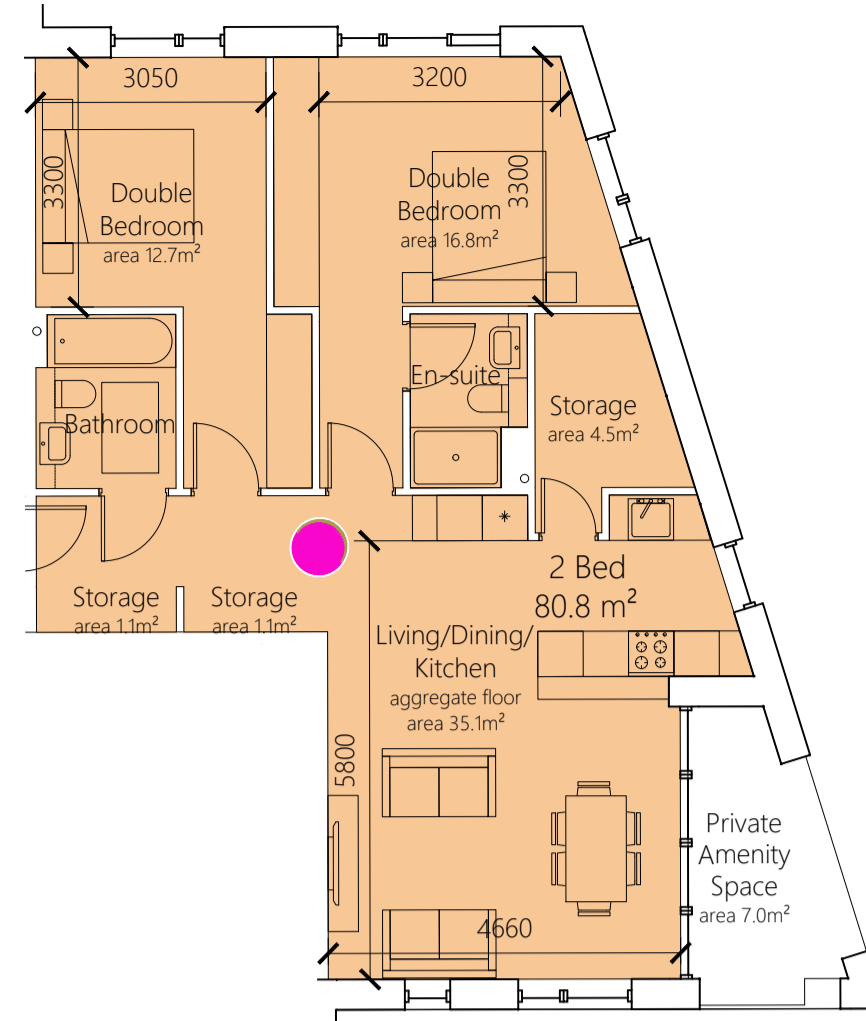
2 BED 4 PERSON i.e. C.0.2 C.1.6 C.2.13 C.3.21 TYPE: 2B4P L AREA: 80.8 m 2
