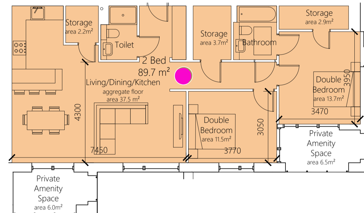
2 BED 4 PERSON i.e. A.5.46 A.6.50 A.7.54 TYPE: 2B4P T AREA: 89.7 m 2
