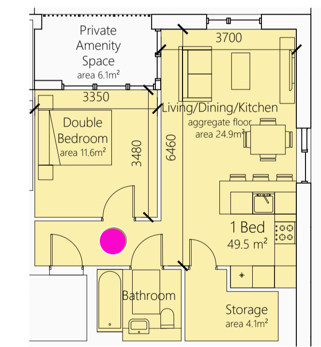
1 BED 2 PERSON i.e. A.5.45, A.6.49, A.7.53, A.8.57 TYPE: 1B2P J AREA: 49.5 m 2
