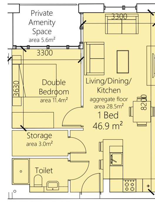
1 BED 2 PERSON i.e. C.0.1, C.1.5, C.2.12, C.3.20 TYPE: 1B2P A2 AREA: 46.9 m 2
