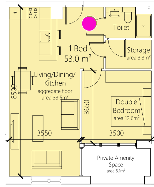
1 BED 2 PERSON i.e. A.1.8, A.2.19, A.3.30, A.4.41 TYPE: 1B1P A1 AREA: 53.0 m 2
