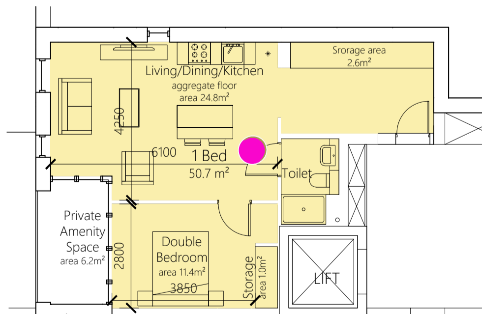
1 BED 2 PERSON i.e. B.3.17, TYPE: 1B2P G AREA: 50.7 m 2
