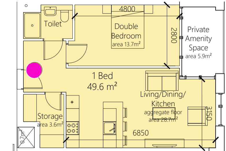
1 BED 2 PERSON i.e. B.1.8, B.2.14 TYPE: 1B2P B1 AREA: 49.6 m 2
