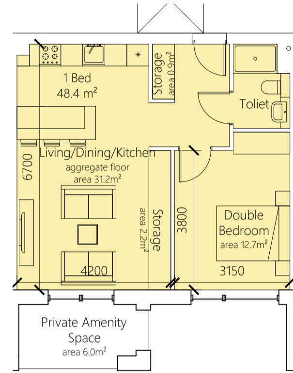
1 BED 2 PERSON i.e. A.1.6, A.1.9, A.2.17, A.2.20 TYPE: 1B2P C AREA: 48.4 m 2
