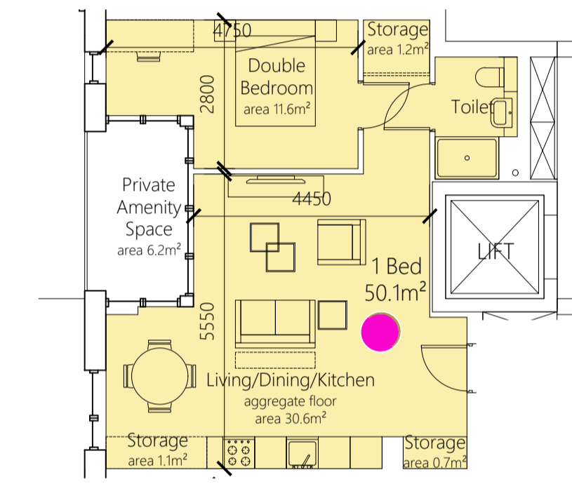
1 BED 2 PERSON i.e. B.1.5 TYPE: 1B2P F AREA: 50.1 m 2
