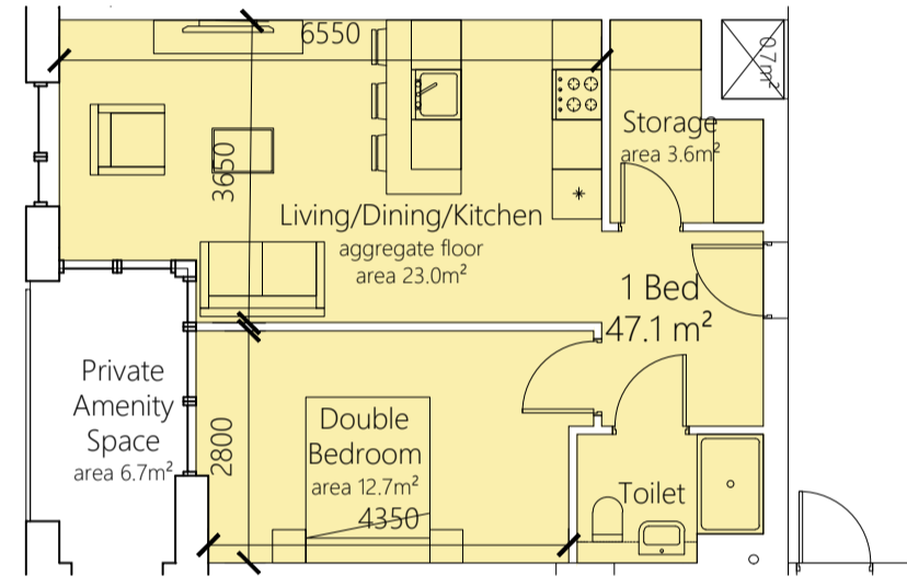
1 BED 2 PERSON i.e. D.0.1, D.0.4, D.1.5, D.1.11 TYPE: 1B2P B2 AREA: 47.1 m 2
