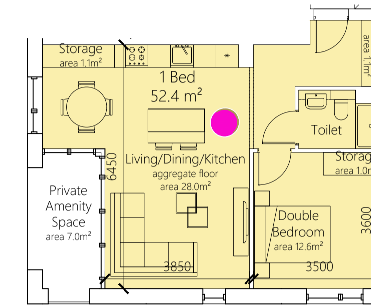
1 BED 2 PERSON i.e. B.0.2, B.1.4 TYPE: B.1.4 E AREA: 52.4 m 2
