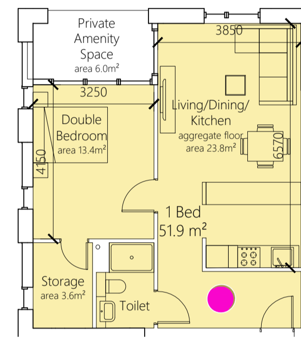
1 BED 2 PERSON i.e. A.1.11, A.2.22, A.3.33, A.4.44 TYPE: 1B2P D AREA: 51.9 m 2
