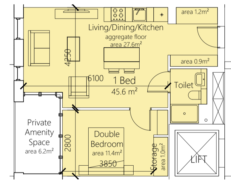
1 BED 2 PERSON i.e. B.2.11, D.2.16, D.3.24 TYPE: 1B2P H AREA: 45.6 m 2
