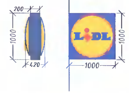
SIGN TYPE 1 - 1 NO. BRACKET FIXED LOGO SIGNAGE (1m X 1m) SCALE: 1:100
