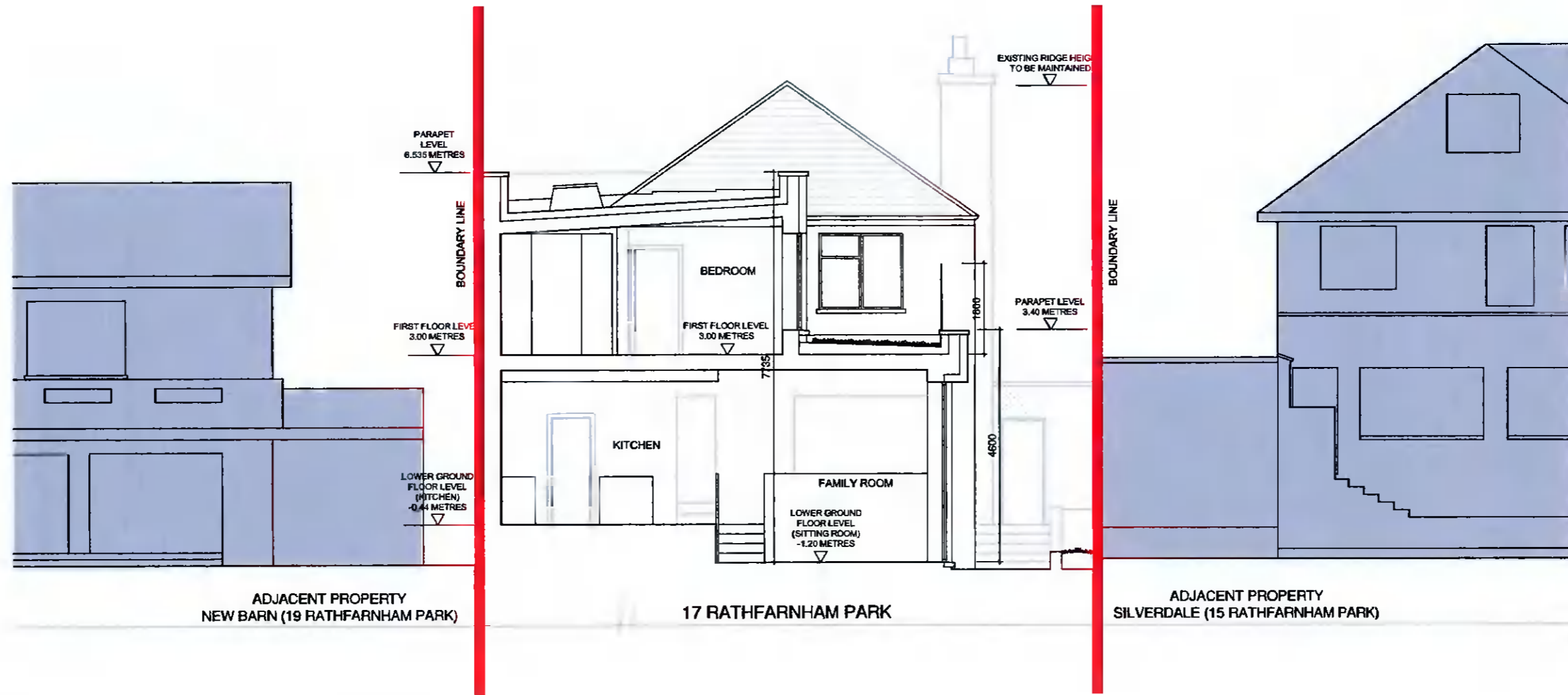
PROPOSED CROSS SECTION (B-B), Scale: 1/100
