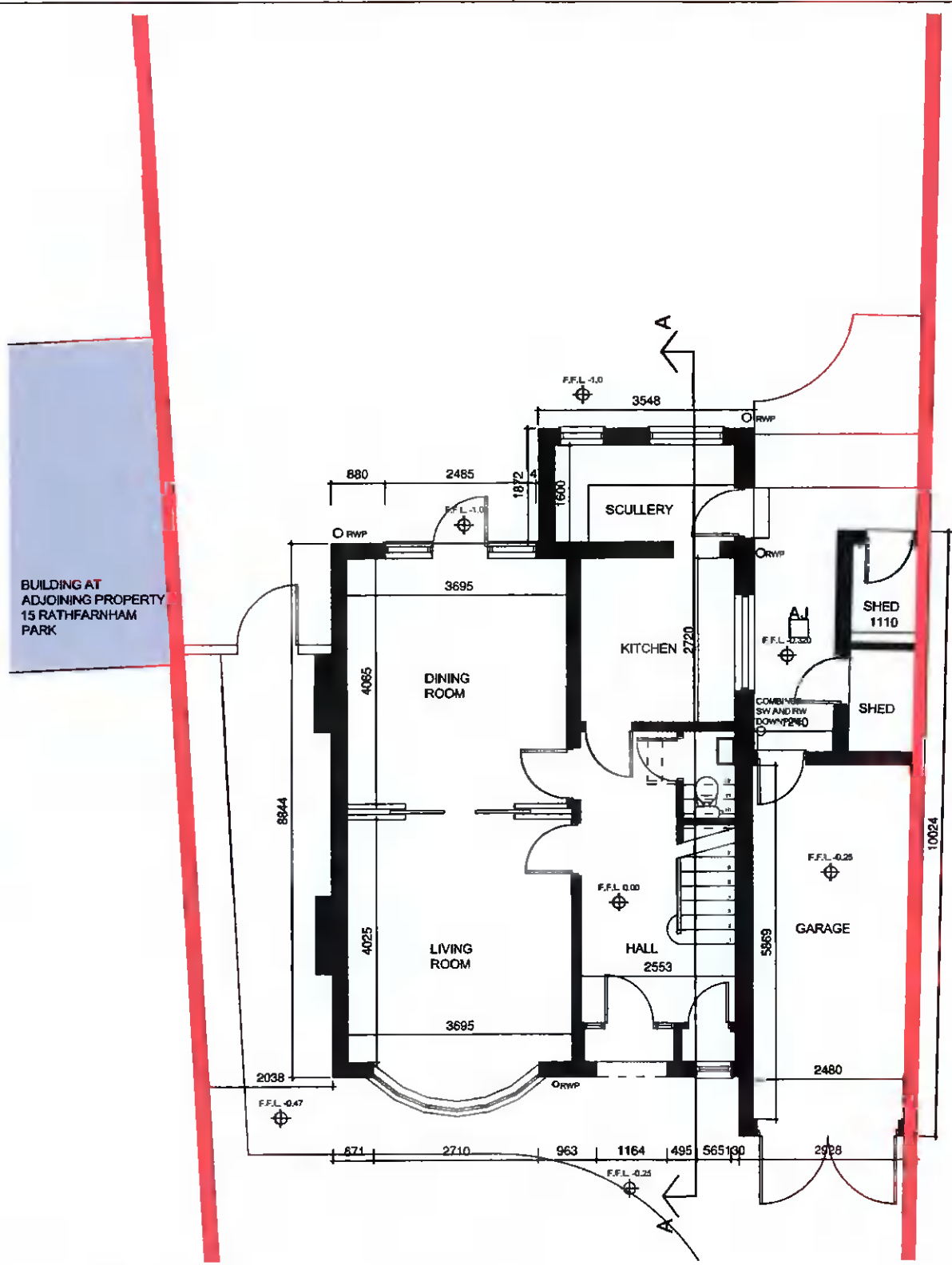
EXISTING GROUND FLOOR PLAN, Scale: 1/100 Current area: 79 sqm
