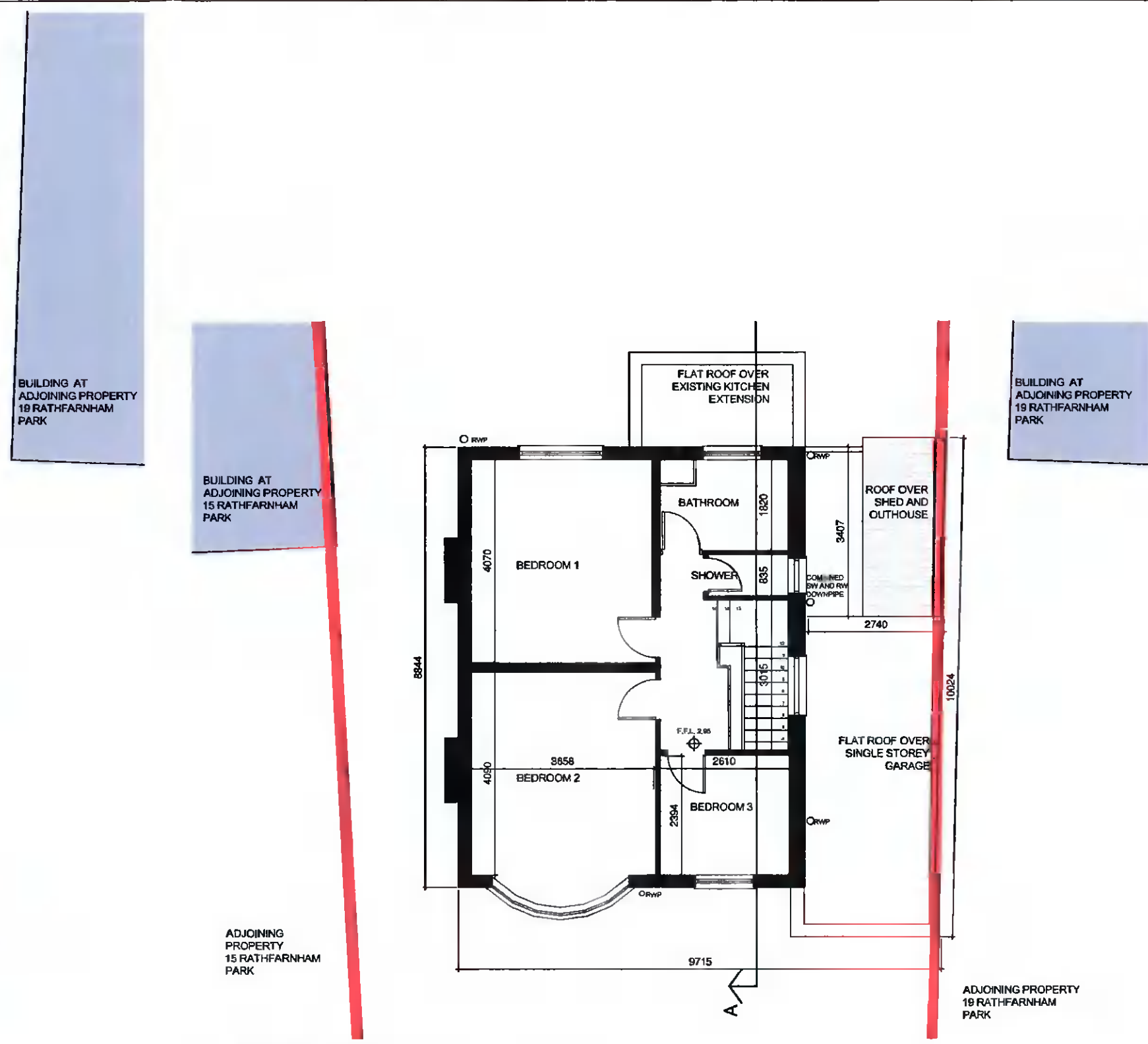
EXISTING FIRST FLOOR PLAN, Scale: 1/100 Current area: 54 sqm
