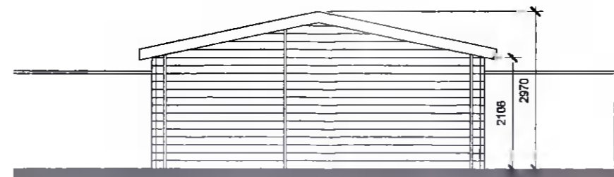
West Elevation 1 : 100
