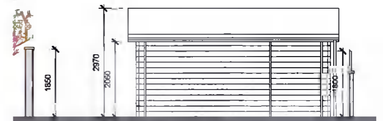
North Elevation 1 : 100
