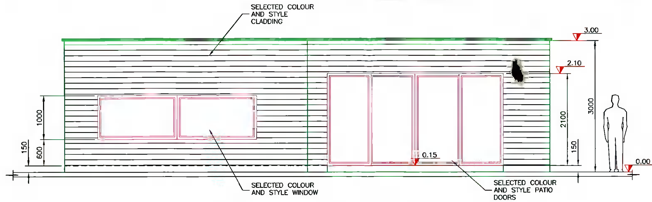
1-1 - PROPOSED ELEVATION
