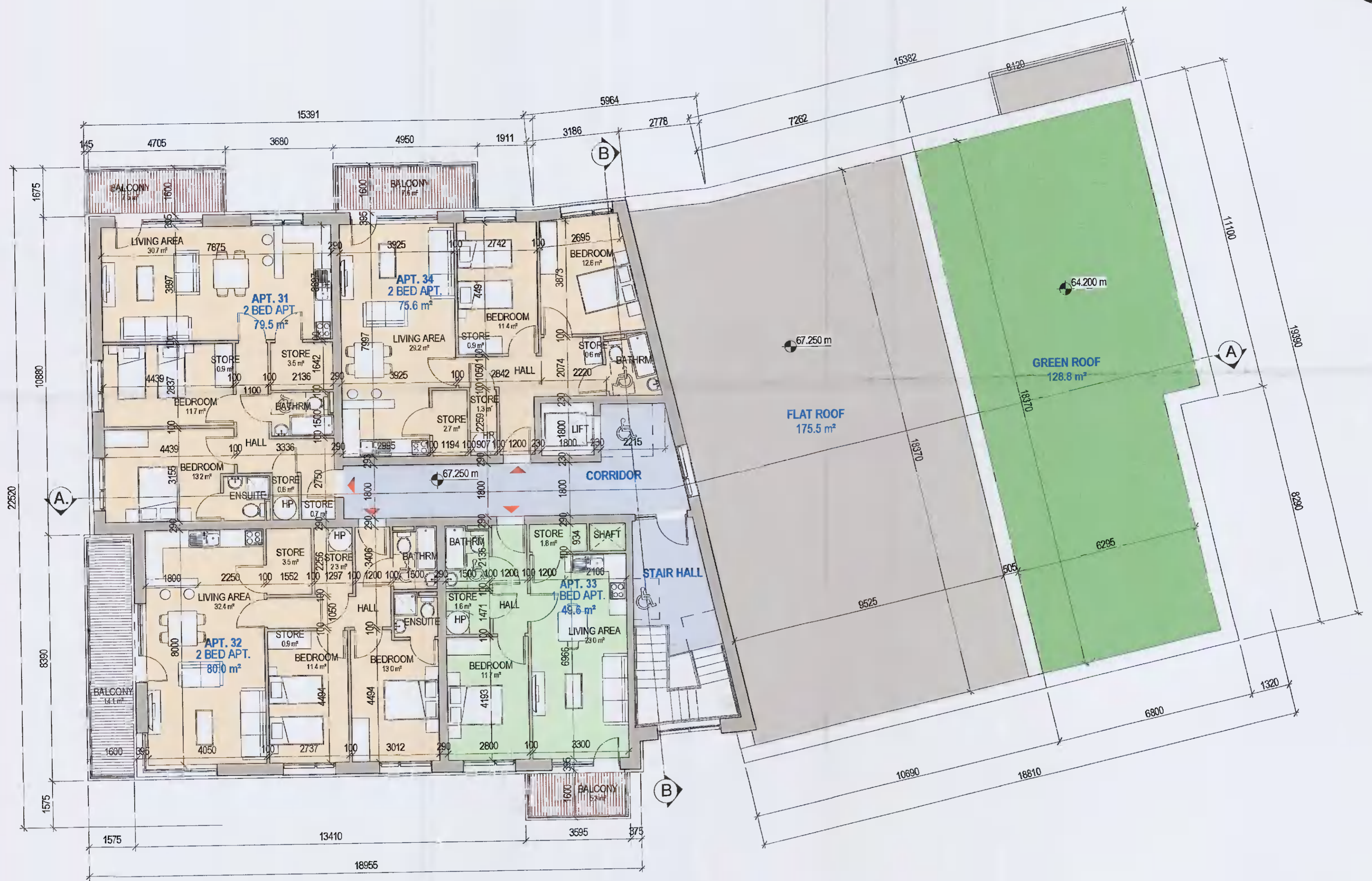
BLOCK 3 FOURTH FLOOR PLAN 1 : 100
