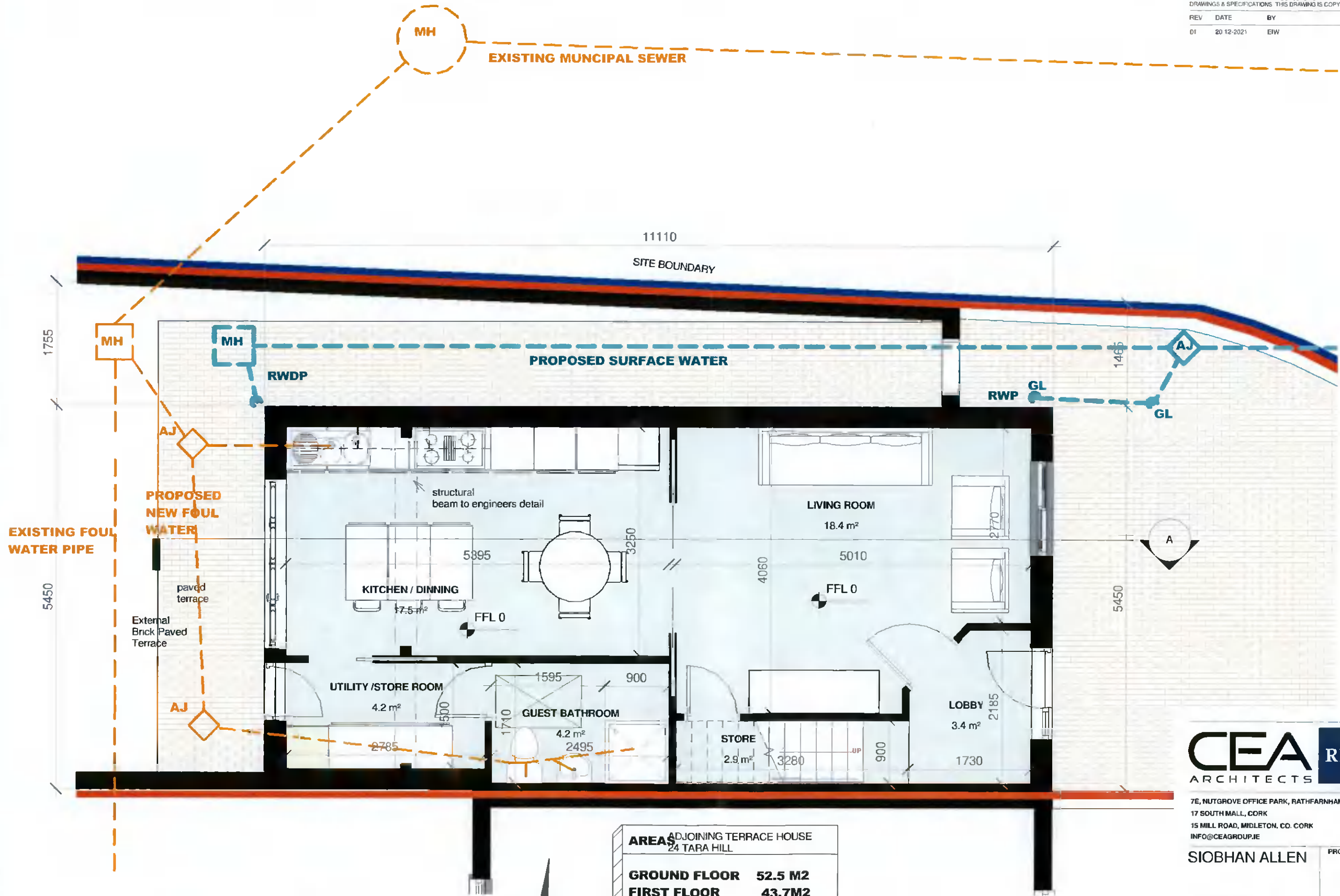
1 GROUND FLOOR PLAN 1 : 50
