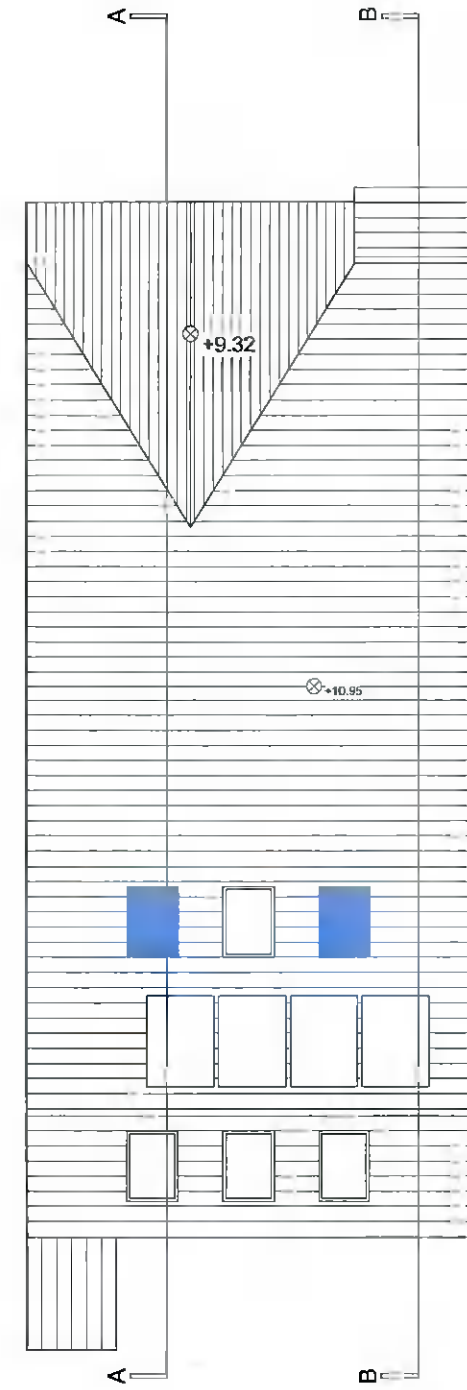
EXISTING ROOF PLAN 1:100
