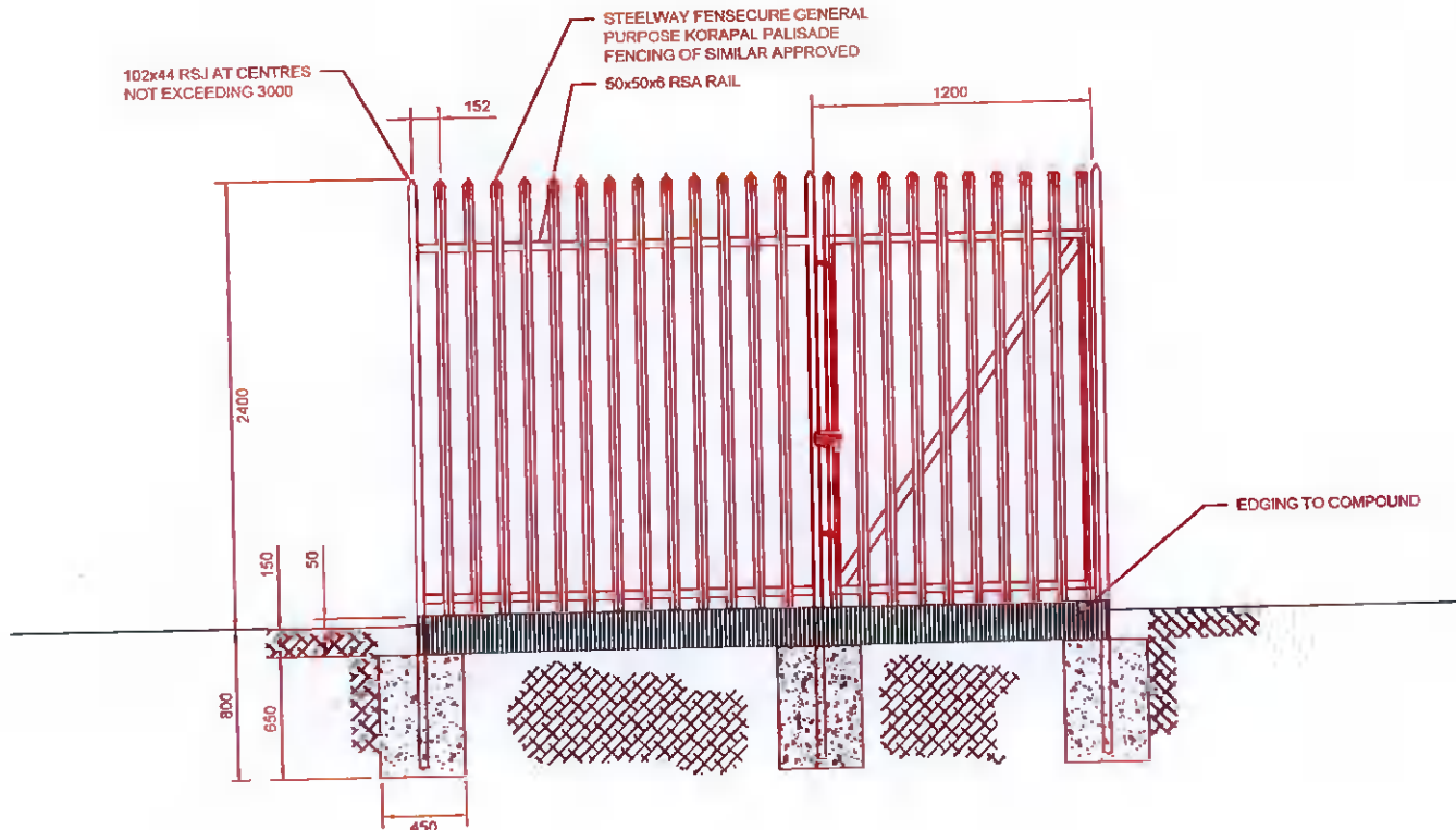
TYPICAL ENCLOSURE PALISADE FENCE DETAIL 1:30 OF ESB TELECOMS COMPOUND FOR RETENTION
