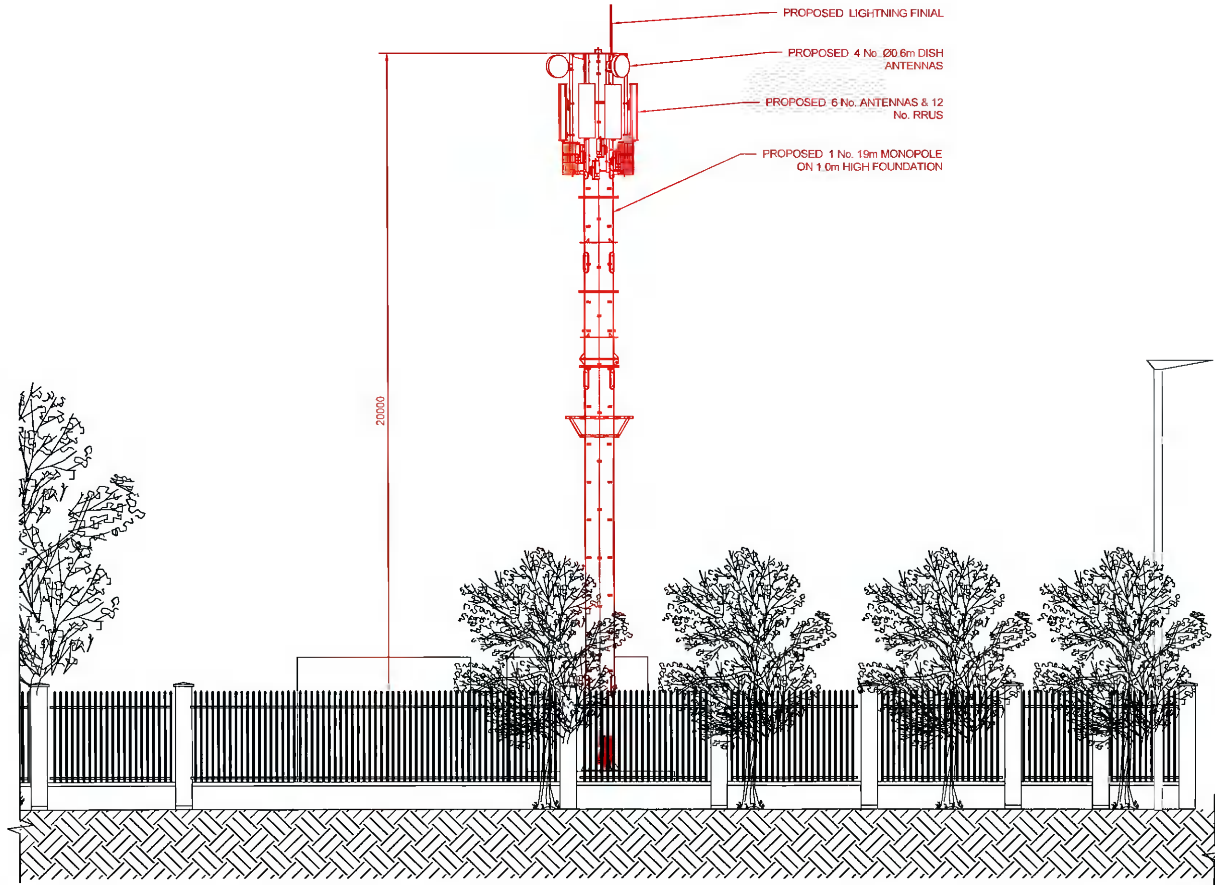
NORTH ELEVATION 4 1:100 103
