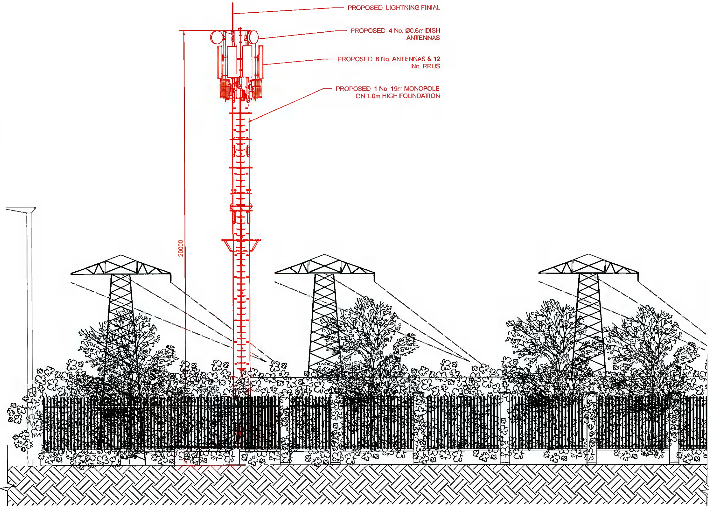
EAST ELEVATION 3 1:100 103
