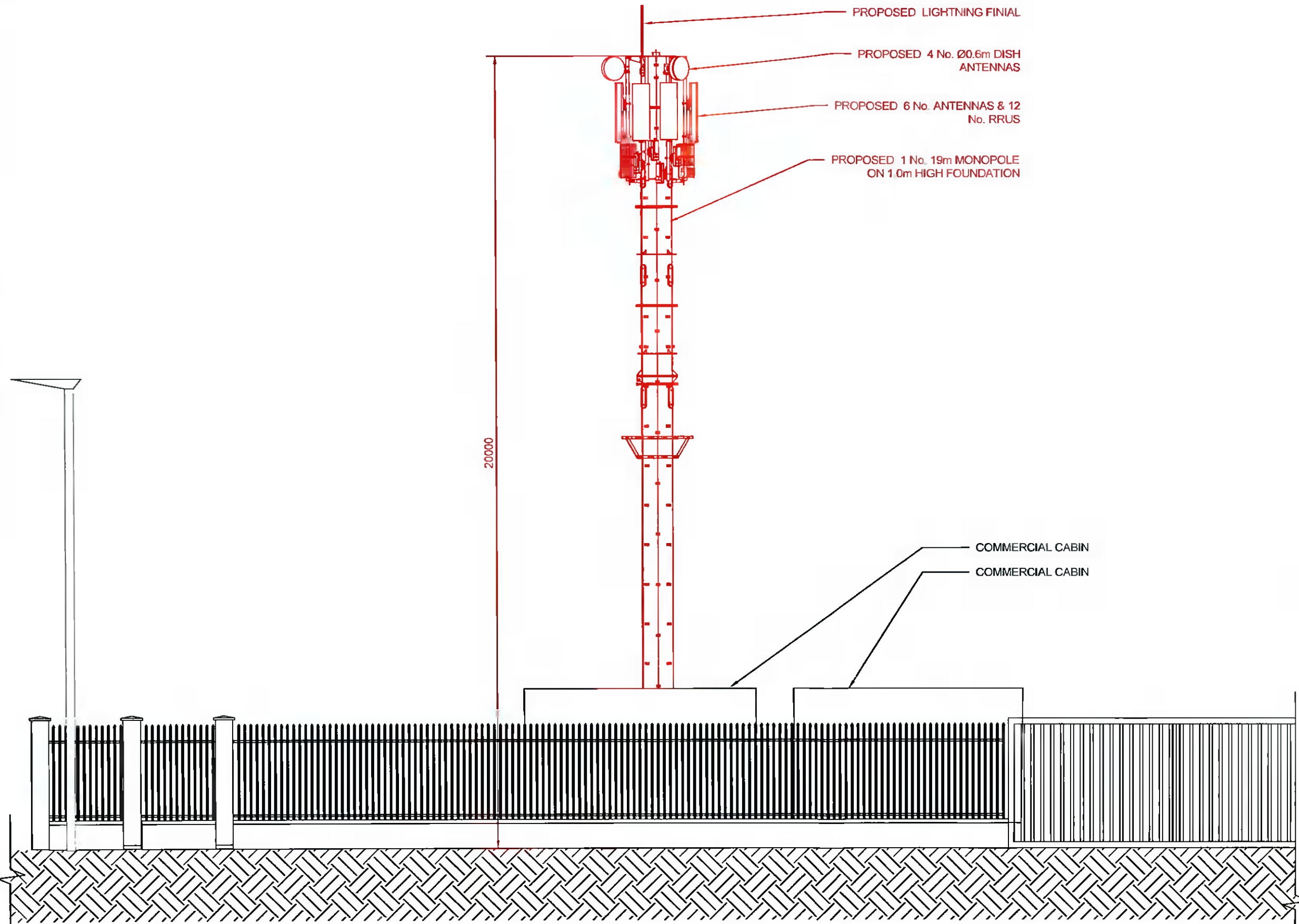
SOUTH ELEVATION 2 1:100 103
